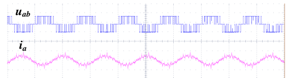
(c) Results of BBCS synchronous SVPWM
