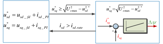
Fig. 5. Switching control strategy
