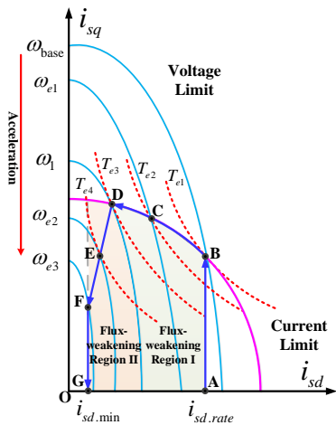
Fig. 4. Working areas of IM
