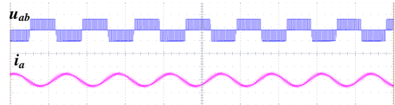
(b) Results of asynchronous SVPWM
