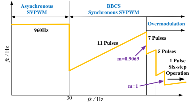
(a) PWM scheme
