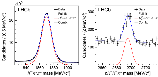
FIG. 1. Invariant-mass distributions for (left) D^+ candidates in B \rightarrow D^+ \mu^- \bar{\nu}_\mu X decays and (right) \Omega_c^0 candidates in \Omega_c^0 \mu^- \bar{\nu}_\mu X decays. The results of the fits, as described in the text, are overlaid.
