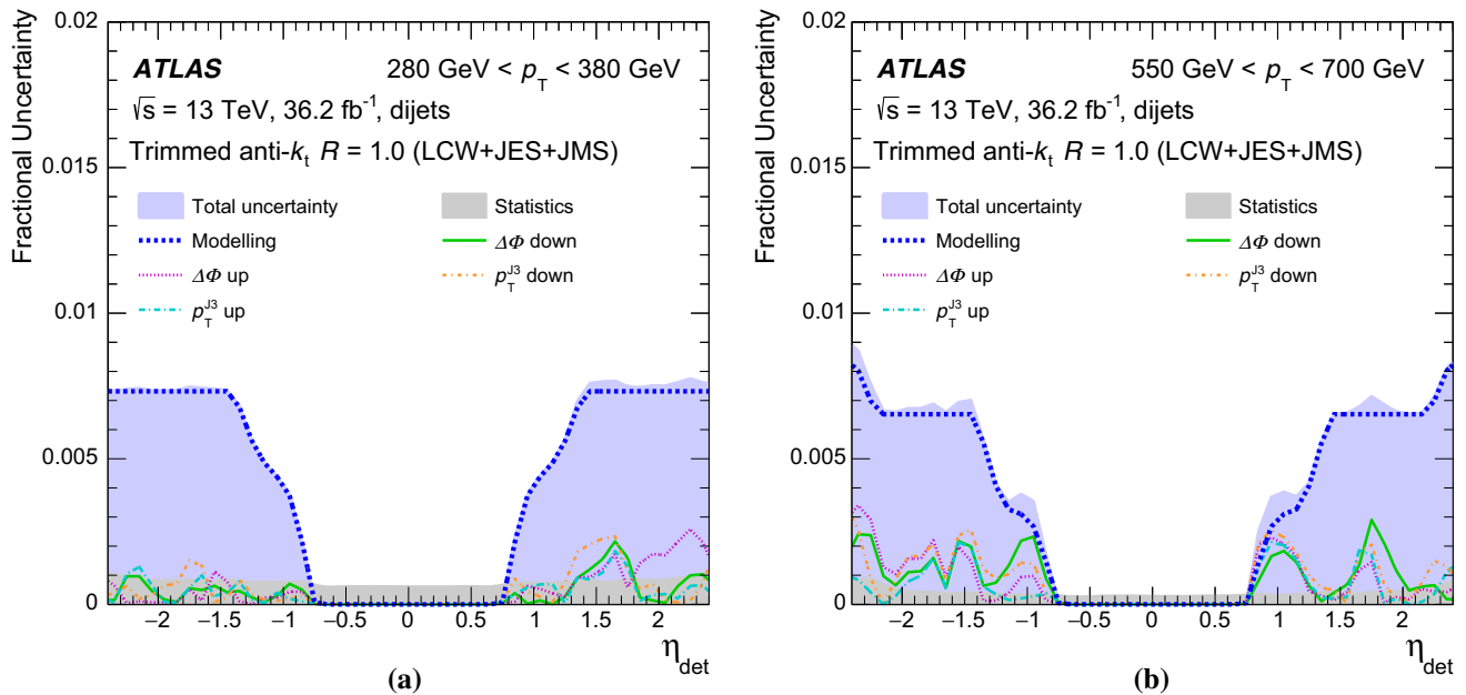
Fig. 6 Uncertainties associated with the large- R jet \eta -intercalibration as a function of detector pseudorapidity \eta_{\text{det}} in two representative average transverse momentum p_T^{\text{avg}} bins a 280 \text{ GeV} < p_T^{\text{avg}} < 380 \text{ GeV} and b 550 \text{ GeV} < p_T^{\text{avg}} < 700 \text{ GeV} . The uncertainties evaluated
