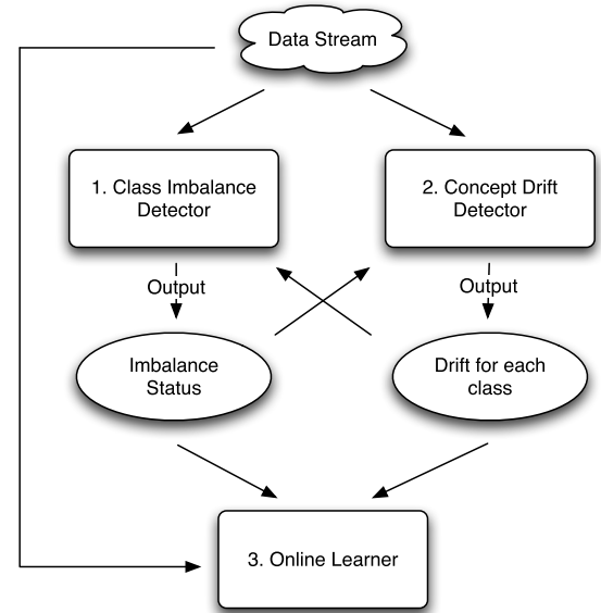
Fig. 1. Learning framework for online class imbalance learning [20].
