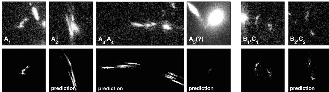
FIG. 2.— V + I -based color renditions of the observed lensed sources ( top row ) compared with the corresponding model-generated images in the bottom row . The leftmost image of each source is the template used to predict the structure of the other counterimages. [See the electronic edition of the Journal for a color version of this figure.]
