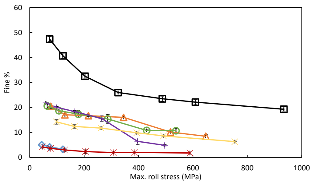
Figure 9. The amount of fines (w/w%) produced for the powder feeds with the unlubricated smooth rollers as a function of the maximum roll stress. The symbols for the powder feeds correspond to: \text{CaCO}_3 (□), mannitol (Δ), lactose 200M (○), anhydrous lactose (+), starch (x), maltodextrin (◇) and MCC (*).
