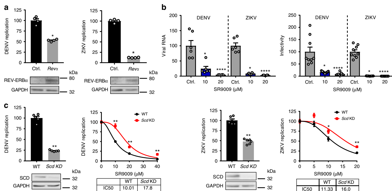
Fig. 6 REV-ERB inhibits DENV and ZIKV replication. a Overexpressing REV-ERB \alpha inhibits DENV and ZIKV replication. Huh-7 cells harbouring sub-genomic DENV RNA or ZIKV-Nanoluc were transfected with REV-ERB \alpha expression plasmid or Ctrl empty vector (2 \mu g). DENV or ZIKV replication was assessed by measuring luciferase activity 48 h later and data expressed relative to untreated Ctrl cells (mean \pm S.E.M., n = 4 , Mann-Whitney statistical test). REV-ERB expression was confirmed by western blotting. b REV-ERB agonist SR9009 inhibits DENV and ZIKV infection. Huh-7 cells were infected with DENV2 16681 at a MOI of 0.1 and treated with SR9009 for 48 h ( n = 3 ). Extracellular viral RNA and the infectious titre of secreted virus was quantified and the data expressed relative to untreated Ctrl cells, where the mean titre of virus secreted from untreated cells was 1.6 \times 10^5 pfu/ml. Huh-7 cells were infected with ZIKV MP1751 at an MOI of 0.1 and treated with SR9009 for 48 h. Extracellular RNA and infectious titre was quantified and the data expressed relative to untreated cells, where the mean titre of virus secreted from untreated cells was 2.9 \times 10^6 pfu/ml. c A role for SCD in REV-ERB agonist inhibition of DENV and ZIKV replication. DENV replicon cells or ZIKV-Nanoluc infected cells were transfected with CRISPRs targeting exons 2 and 3 of SCD or a scrambled guide RNA and 24 h later treated with SR9009. SCD expression was measured by western blotting and the dose of REV-ERB agonist required to inhibit DENV or ZIKV replication by 50% (IC 50 ) in WT or KD cells determined (mean \pm S.E.M., n = 6 , Mann-Whitney statistical test)
