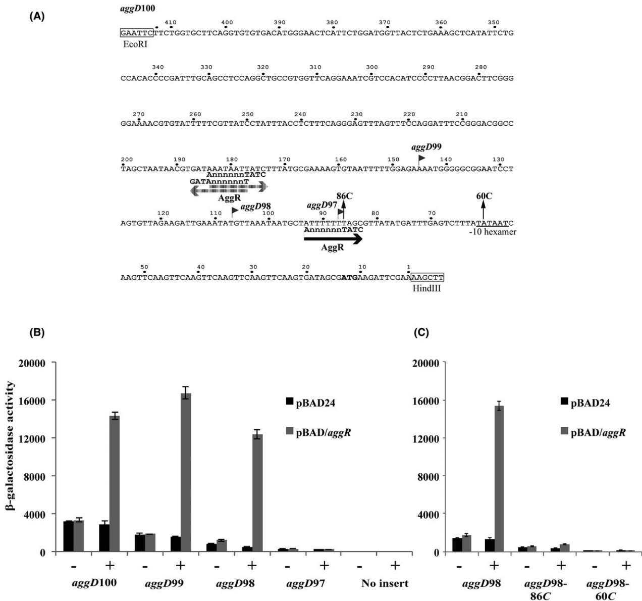
Fig. 4. Analysis of aggD100 promoter fragment from EAEC strain 17-2.
