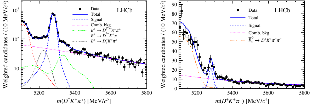
FIG. 2. Weighted invariant mass distribution of candidates in the (left) B^+ \rightarrow D^- K^+ \pi^+ and (right) B^+ \rightarrow D^+ K^+ \pi^- data samples. Data points and fit functions are weighted as described in the text. The components are as detailed in the legend.
