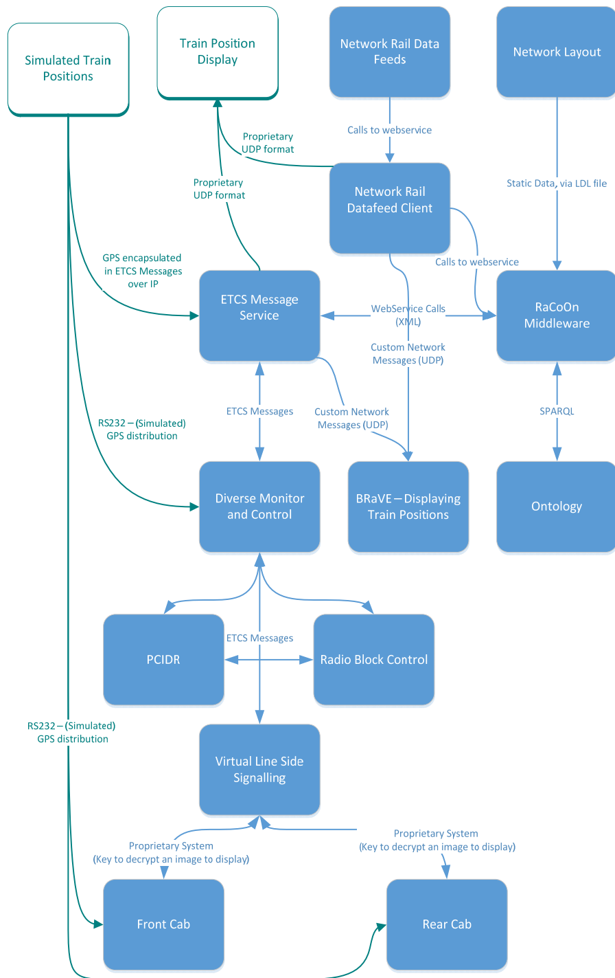
Figure 1 Full System architecture
