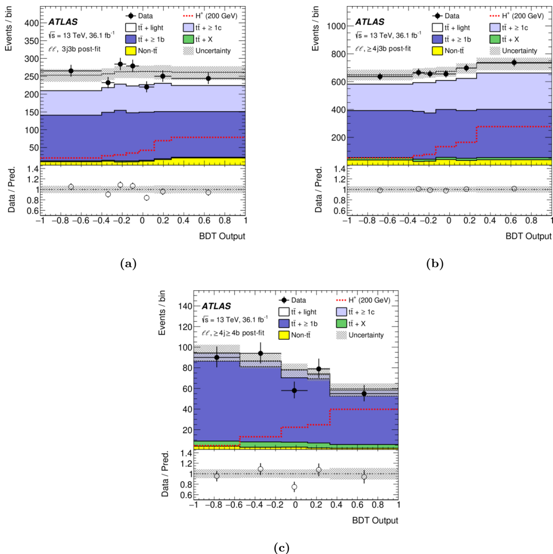
Figure 7. Distributions of the BDT output after the fit to the data in the three SRs of the \ell\ell final state: (a) 3j3b, (b) \geq 4j3b and (c) \geq 4j\geq 4b for the 200 GeV mass hypothesis. Each background process is normalised according to its post-fit cross-section. The t\bar{t} + X includes contributions from t\bar{t}W , t\bar{t}Z and t\bar{t}H . The total prediction of the BDT distributions includes cases where the signal obtained from the fit is negative. For this particular mass point the fitted signal strength is \mu = -0.4 \pm 1.5 pb. The pre-fit signal distribution is shown superimposed as a dashed line with arbitrary normalisation. The lower panels display the ratio of the data to the total prediction. The hatched bands show the post-fit uncertainties.
