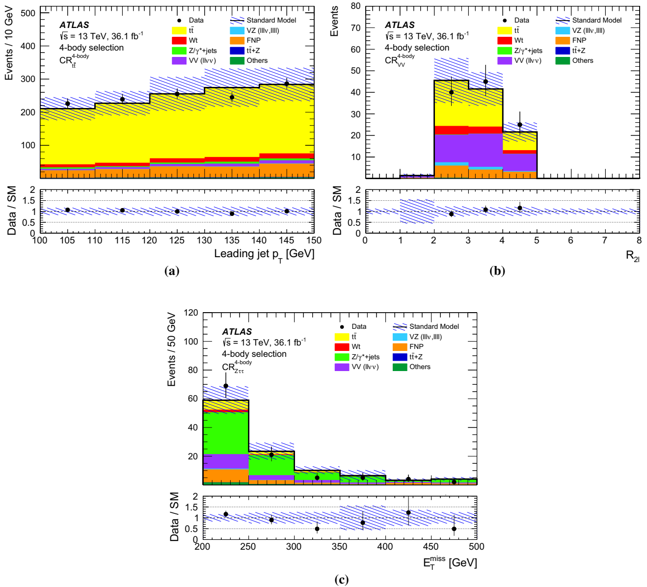
Fig. 4 Four-body selection distributions of the a p_T(j_1) in CR_{t\bar{t}}^{4-body} , b R_{2\ell} in CR_{VV}^{4-body} and c E_T^{miss} in CR_{Z\tau\tau}^{4-body} after the background fit. The contributions from all SM backgrounds are shown as a histogram stack; the hatched bands represent the total uncertainty
