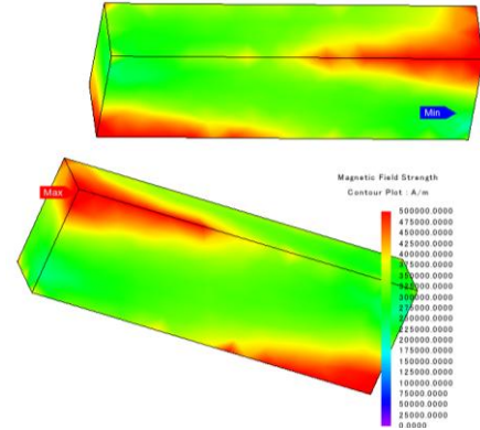
Fig. 13. Demagnetization of virgin magnets at I_d = -325 A and I_q = 0 A
