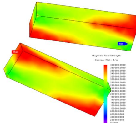
Fig. 15. Demagnetization of recycled magnets at I_d = -325 A and I_q = 0 A
