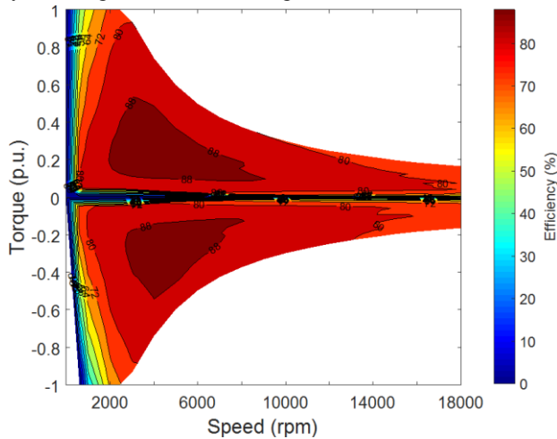
Fig. 9. Efficiency map of the machine with recycled magnets
