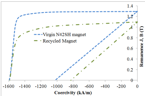
Fig. 5. Measured magnetization BH curve of virgin N42SH and recycled magnet at 25 °C temperature
