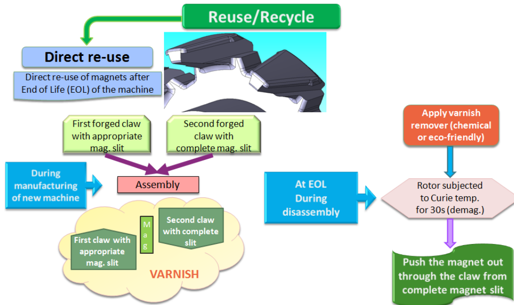
Fig. 2. Direct reuse methodology for assembly and disassembly of magnets in claw-pole machine
