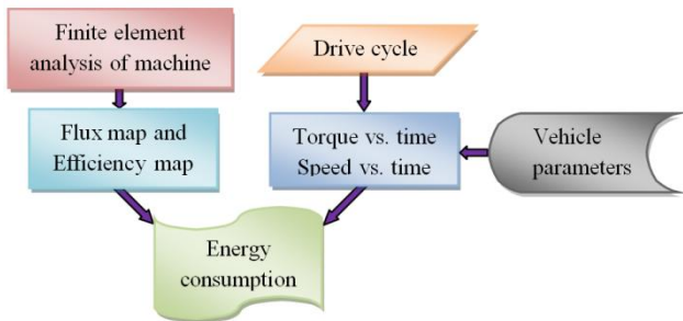
Fig. 8. Flow diagram for energy evaluation methodology [9]
