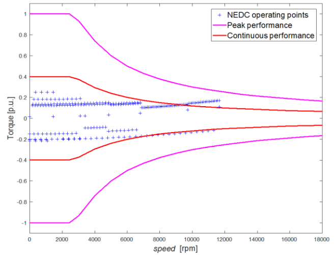
Fig. 11. Torque-speed envelop of the machine with NEDC operating points
