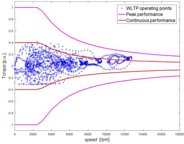
Fig. 12. Torque-speed envelop of the machine with WLTP operating points
