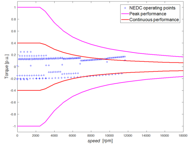
Fig. 11. Torque-speed envelop of the machine with NEDC operating points
