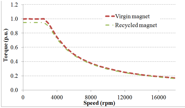
Fig. 7. Torque-speed curve at peak performance with virgin and recycled magnets for the PM based claw-pole machine
