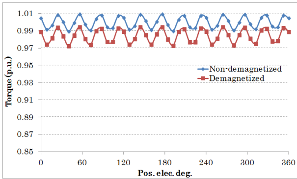
Fig. 16. Developed torque with non-demagnetized & demagnetized recycled PMs
