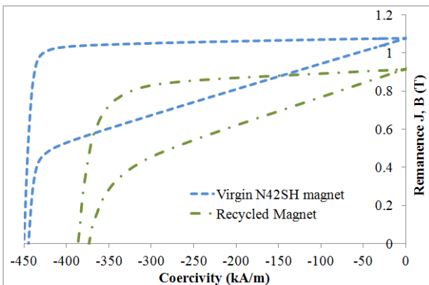
Fig. 6. Measured magnetization BH curve of virgin N42SH and recycled magnet at 150 °C temperature
