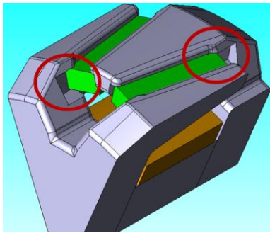
Fig. 1. Claw-poles and magnets with the appropriate magnet slit
