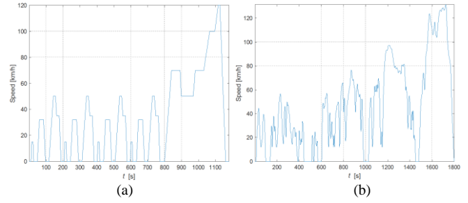
Fig. 10. (a) NEDC drive cycle (b) WLTP drive cycle
