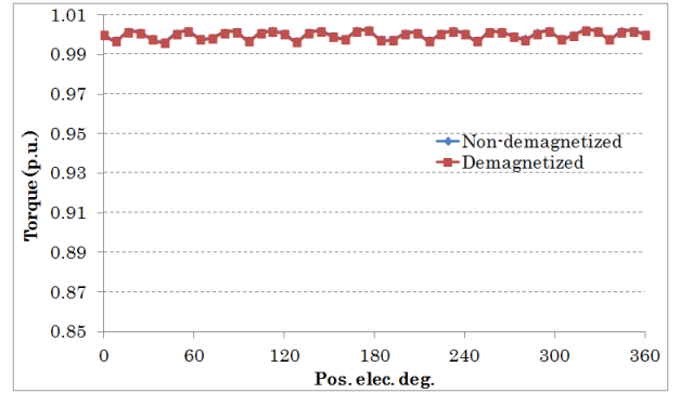
Fig. 14. Developed torque with non-demagnetized & demagnetized virgin PMs
