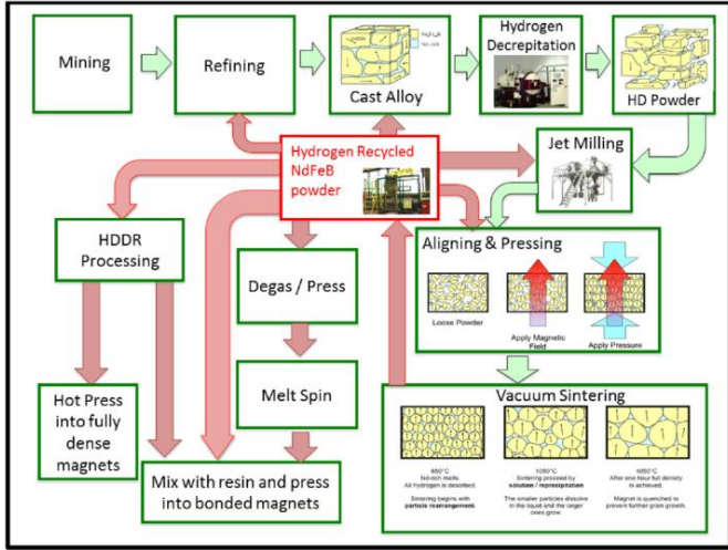
Fig. 4. Schematic of possible re-processing routes. Green boxes show primary route for manufacturing a sintered NdFeB magnet. Red boxes and arrows demonstrate where the hydrogen extracted powder can be fed back in to recycle the material [4]
