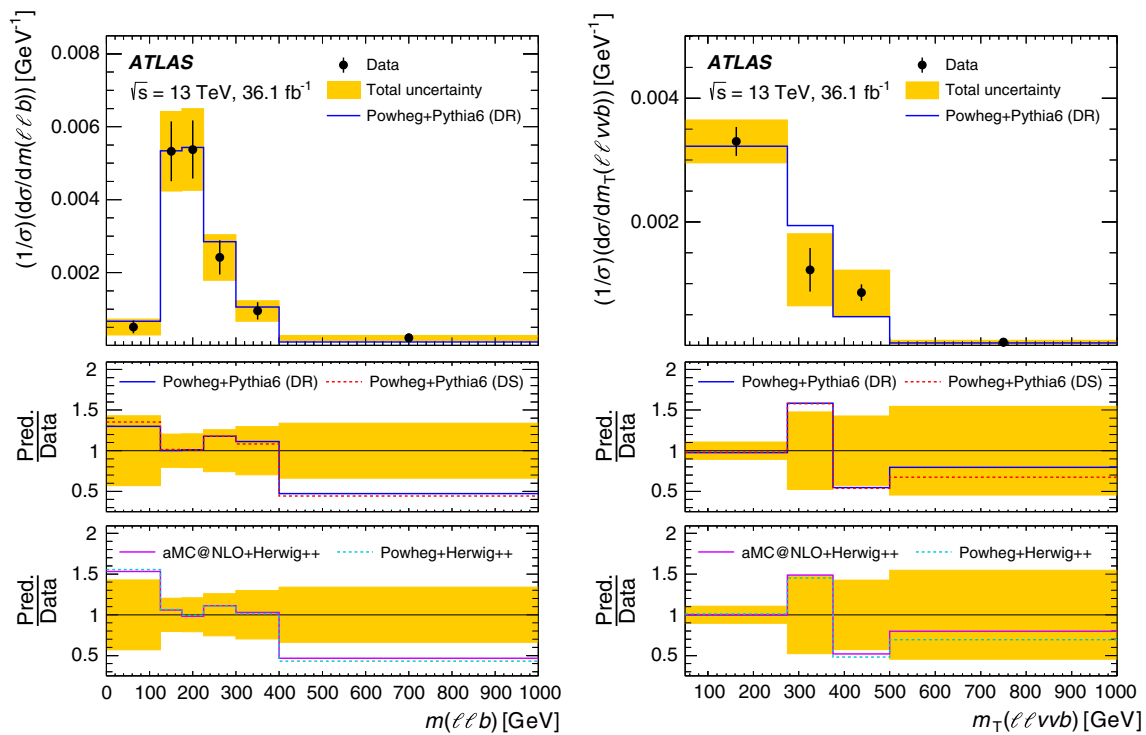
Fig. 6 Normalised differential cross-sections unfolded from data, compared with selected MC models, with respect to m_T(\ell\ell\nu b) and m(\ell\ell b) . Data points are placed at the horizontal centre of each bin. See Sect. 1 for a description of the observables plotted
