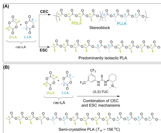
Figure 5. a) Chain-end control (CEC) vs. site enantiomorphic control (ESC) mechanism during the ROP of rac -LA. b) Proposed mechanism using the chiral Takemoto's catalyst, here with a ( S,S ) configuration. Pale blue frames point out the stereoerrors.
