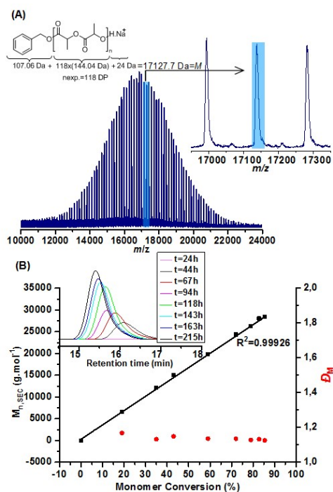
Figure 2. a) MALDI-ToF mass spectrum of PLA obtained at 25 °C (Table 1, entry 2); b) M n,SEC and dispersity ( D M ) vs. monomer conversion for PLA synthesized from ( S,S )-TUC at RT Inset: Size exclusion chromatograms of PLA during ROP (Table 1, entry 2).
