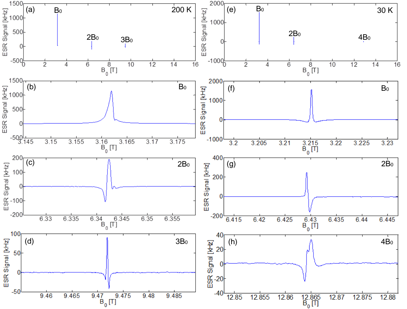
Fig. 7. ESR experiments performed with the 92 GHz single-chip ESR detector with a 6 \times 6 \times 5 \mu\text{m}^3 sample of BDPA at \nu_m = 98 kHz, B_m = 0.12 mT, B_1 \cong 0.2 mT, \Delta f = 0.25 Hz, t_s = 3 min (10 mT/min), T = 200 K, \omega_0 \cong 2\pi \times 92 GHz. (a) All measurements. Narrow field sweeps about (b) B_0 = (\omega_0 / \gamma) , (c) B_0 = 2(\omega_0 / \gamma) , (d) B_0 = 3(\omega_0 / \gamma) , respectively. ESR spectra of a 3 \times 3 \times 3 \mu\text{m}^3 of BDPA (see text) with \nu_m = 98 kHz, B_m = 0.12 mT, B_1 \cong 0.2 mT, \Delta f = 0.25 Hz, t_s = 1 min, T = 30 K. (e) All measurements. Narrow field sweeps about (f) B_0 = (\omega_0 / \gamma) , (g) B_0 = 2(\omega_0 / \gamma) , (h) B_0 = 4(\omega_0 / \gamma) , respectively. Note: signals at B_0 = 4(\omega_0 / \gamma) at 200 K and at B_0 = 3(\omega_0 / \gamma) at 30 K have been also observed but not reported in the graphs above because accidentally measured with a much faster magnetic field sweep rate which reduced their signal amplitude and distorted their shape.
