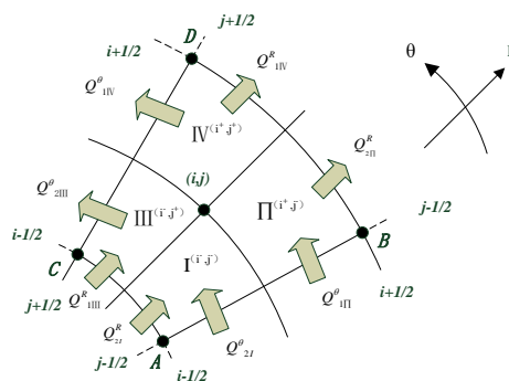
Figure 1. The defined control volume
