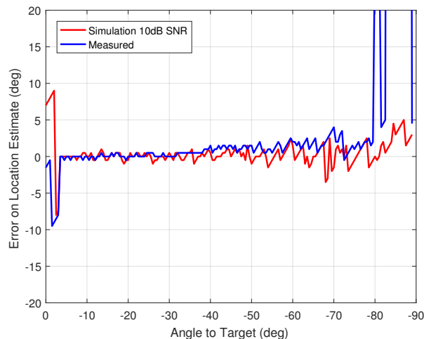
(d) Result for target localisation in azimuth using the phase-based HRTF technique. Simulation results for 10dB SNR are shown in red, and measurement results (with variable SNR) are in blue.
