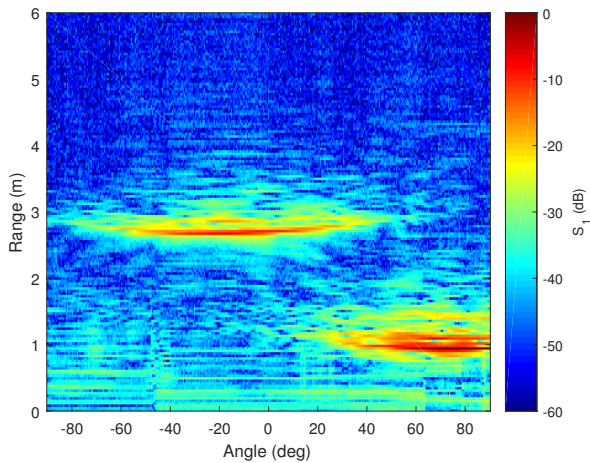
(a) The chamber with the target. Here, clutter is visible at low angles. The clutter at a range of 1m at 20^{\circ} - 90^{\circ} is caused by a pillar that was placed in the corner of the chamber behind the apparatus.
