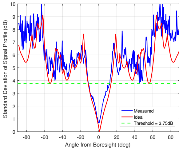
(a) Angular variance, power approach.
