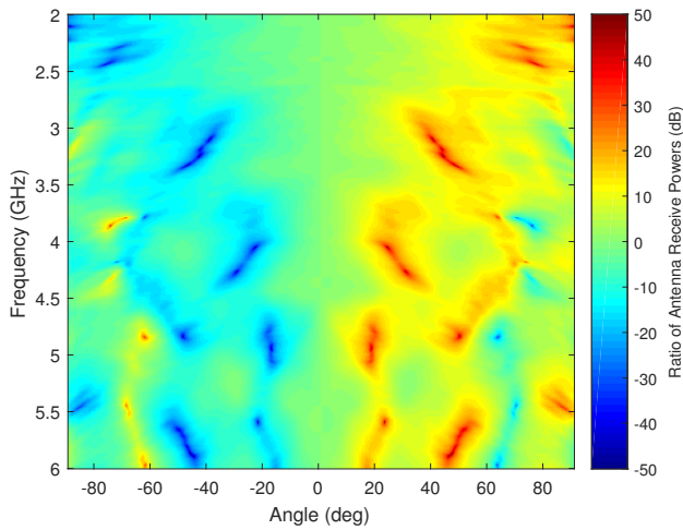
(b) Power map function.
