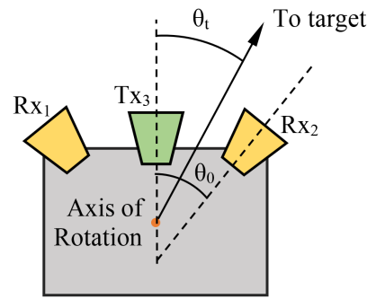
Fig. 4: The biologically-inspired radar configuration.
