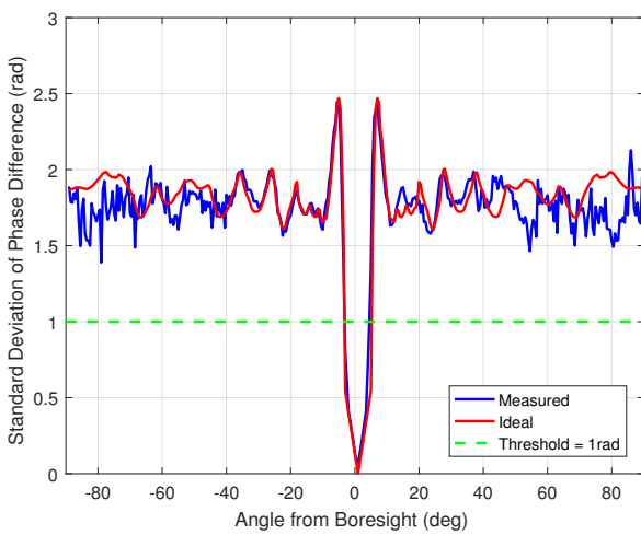
(b) Angular variance, phase approach.
