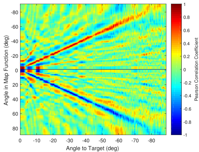
(c) Result of the Pearson correlation between each frequency profile in the map function and the signal phase difference using the phase-based approach.
