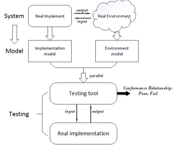
Fig 1 Schematic of conformance testing with MBT
