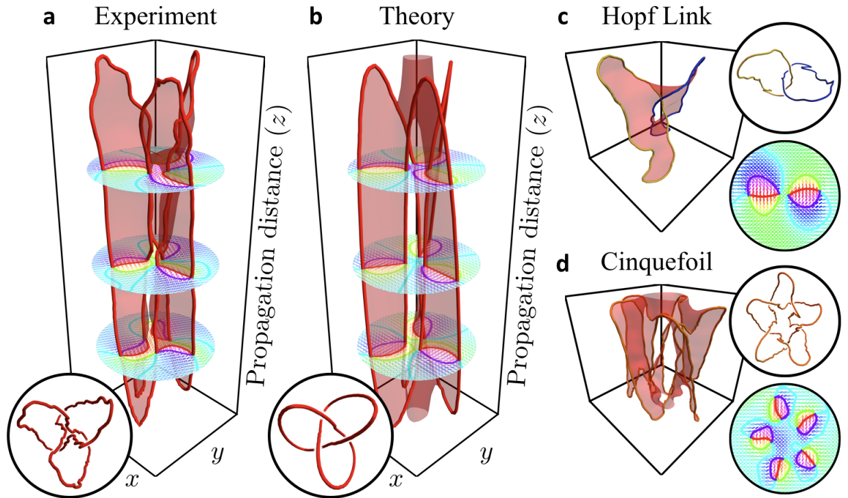
Fig. 2. Topological traits of torus structures. Depiction of the various entities attributed to an optical trefoil knot corresponding to a , experimental and b , theoretical results. In this display, the knotted trajectories of the C-lines are shown in red and the Seifert surface defined by regions
