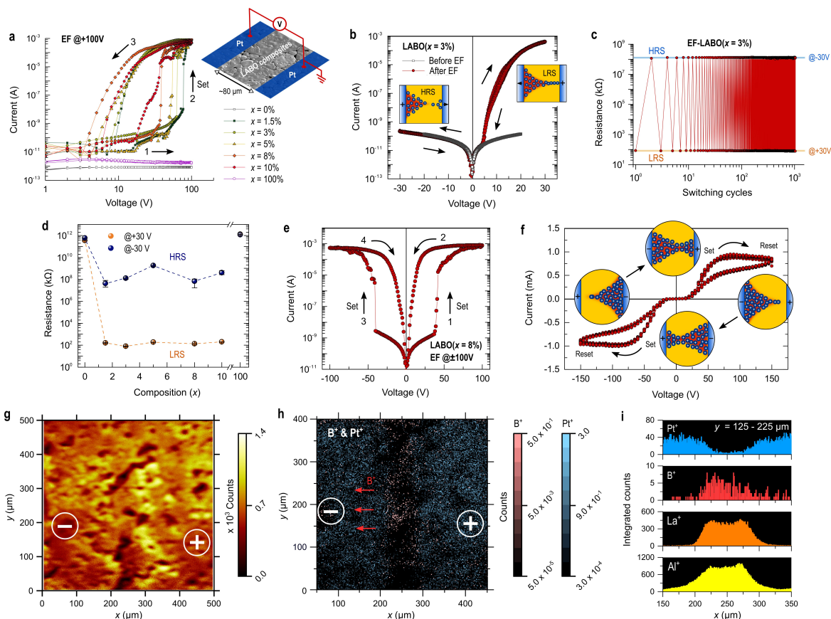
Figure 2. a) Electroforming (EF) process in the undoped LAO, LBO, and LABO( x ) composites after a poling sequence, i.e. 0\text{ V} \rightarrow +100\text{ V} \rightarrow 0\text{ V} , across a gap of 80\ \mu\text{m} . The inset shows a schematic depicting the geometry of DC measurements with planar Pt electrodes separated by a gap of 80\ \mu\text{m} . b) Current-voltage (I-V) curves of the LABO( x = 3\% ) composite before and after the EF process. c) The cyclic switching performance of the low (LRS) and high resistance states (HRS) of the EF-LABO( x = 3\% ) composite upon application of a \pm 30\text{ V} pulse over a period of 10^3 repetition. d) LRS/HRS ratios in the undoped LAO and LBO, and EF-LABO( x ) composites. e) The bipolar switching of the LABO( x = 8\% ) composite by applying hysteric high voltage sweeps of \pm 100\text{V} in a sequence (1 \rightarrow 2 \rightarrow 3 \rightarrow 4). f) 10-time I-V hysteresis curves of the composite, measured at \pm 150\text{ V} at a rate of approximately 12.5\text{ V/sec} after the bipolar switching. The set-and-reset transition of the resistive switching is schematically depicted by a cyclic sequence of field-driven two-filament growth and gap opening during the operation. g) An electrically poled area at the surface of the LABO( x = 8\% ) composite measured by ToF-SIMS. h) 2D elementary mapping of B and Pt ions across the electrode gap. The highlighted dashed area corresponds to the dashed area within the white solid line square given in (g). The maximum scale ranges of \text{B}^+ and \text{Pt}^+ counts are adjusted for visualisation of the B ion distribution across the Pt electrodes. i) The integrated counts of the detected Pt, B, La, and Al ions for the area ( x = 150 - 350\ \mu\text{m} , y = 125 - 225\ \mu\text{m} ).
