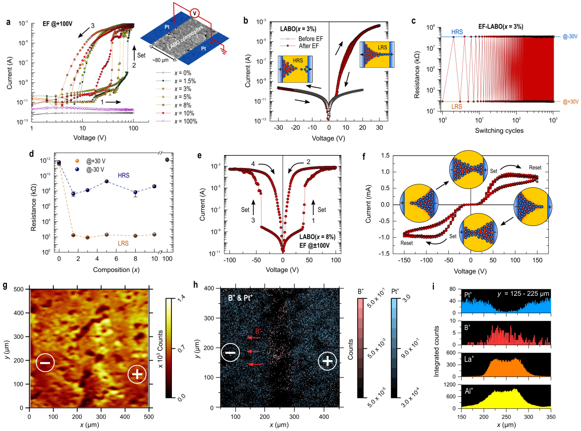
Figure 2. a) Electroforming (EF) process in the undoped LAO, LBO, and LABO( x ) composites after a poling sequence, i.e. 0 V \rightarrow +100 V \rightarrow 0 V, across a gap of 80 \mu m. The inset shows a schematic depicting the geometry of DC measurements with planar Pt electrodes separated by a gap of 80 \mu m. b) Current-voltage (I-V) curves of the LABO( x = 3%) composite before and after the EF process. c) The cyclic switching performance of the low (LRS) and high resistance states (HRS) of the EF-LABO( x = 3%) composite upon application of a \pm 30 V pulse over a period of 10^3 repetition. d) LRS/HRS ratios in the undoped LAO and LBO, and EF-LABO( x ) composites. e) The bipolar switching of the LABO( x = 8%) composite by applying hysteric high voltage sweeps of \pm 100V in a sequence (1 \rightarrow 2 \rightarrow 3 \rightarrow 4). f) 10-time I-V hysteresis curves of the composite, measured at \pm 150 V at a rate of approximately 12.5 V/sec after the bipolar switching. The set-and-reset transition of the resistive switching is schematically depicted by a cyclic sequence of field-driven two-filament growth and gap opening during the operation. g) An electrically poled area at the surface of the LABO( x = 8%) composite measured by ToF-SIMS. h) 2D elementary mapping of B and Pt ions across the electrode gap. The highlighted dashed area corresponds to the dashed area within the white solid line square given in (g). The maximum scale ranges of B ^{+} and Pt ^{+} counts are adjusted for visualisation of the B ion distribution across the Pt electrodes. i) The integrated counts of the detected Pt, B, La, and Al ions for the area ( x = 150 - 350 \mu m, y = 125 - 225 \mu m).
