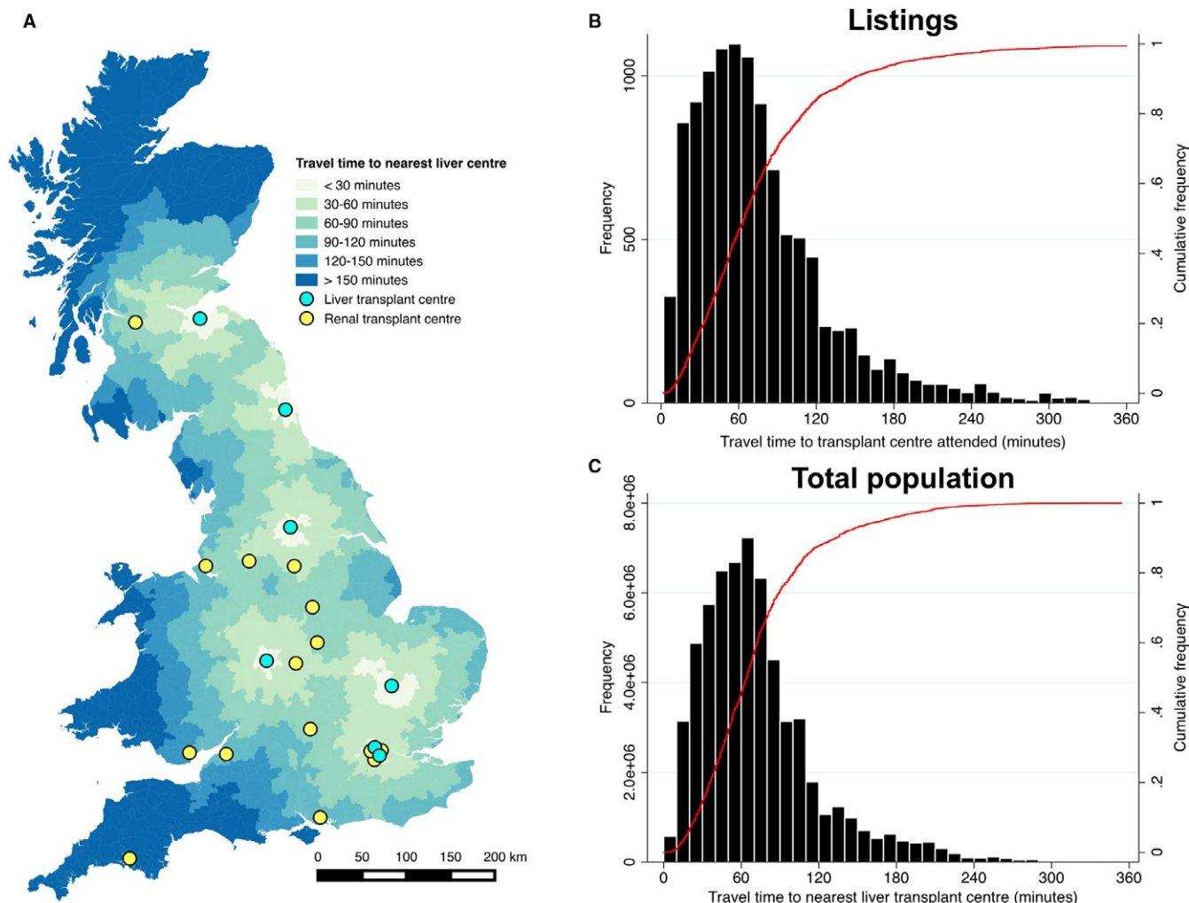
FIGURE 4 Travel time to nearest liver transplant center. A, Map of Great Britain showing the locations of current liver transplant centers (cyan circles), renal transplant centers without liver transplant capability (yellow circles), and calculated travel time to the nearest liver transplant center from each postcode district in 30-minute intervals. B, Frequency distribution of travel time from postcode district of residence of patients listed for transplantation to the liver transplant center attended ( n = 11\,188 ). Red line denotes cumulative frequency. C, Frequency distribution of travel time from postcode district of residence of total resident population to the nearest liver transplant center ( n = 6.13 \times 10^7 ). Red line denotes cumulative frequency
