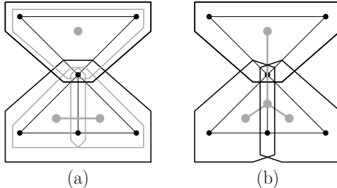
FIGURE 2. (a) shows the tree-decomposition \mathcal{T} of G , drawn in black, and the tree-decompositions of the torsos, drawn in grey. (b) shows the canonically glued tree-decomposition \overline{\mathcal{T}} .
