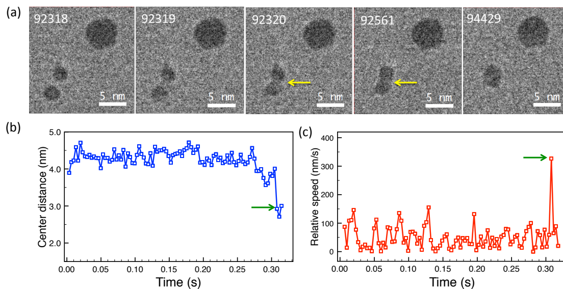
Figure 2 (a) Coalescence between two \text{Au}_{923} clusters (bottom left). The frame number is labelled on the top left corner of each image and the time interval between each frame is 3.31 ms. The yellow arrows indicate the “neck” formation. (b) Center-to-center distance versus time, and (c) relative speed changing of the two clusters versus time. The distance and relative speed were measured from frame 92220 to 92320. The contacting points are indicated by the green arrows.
