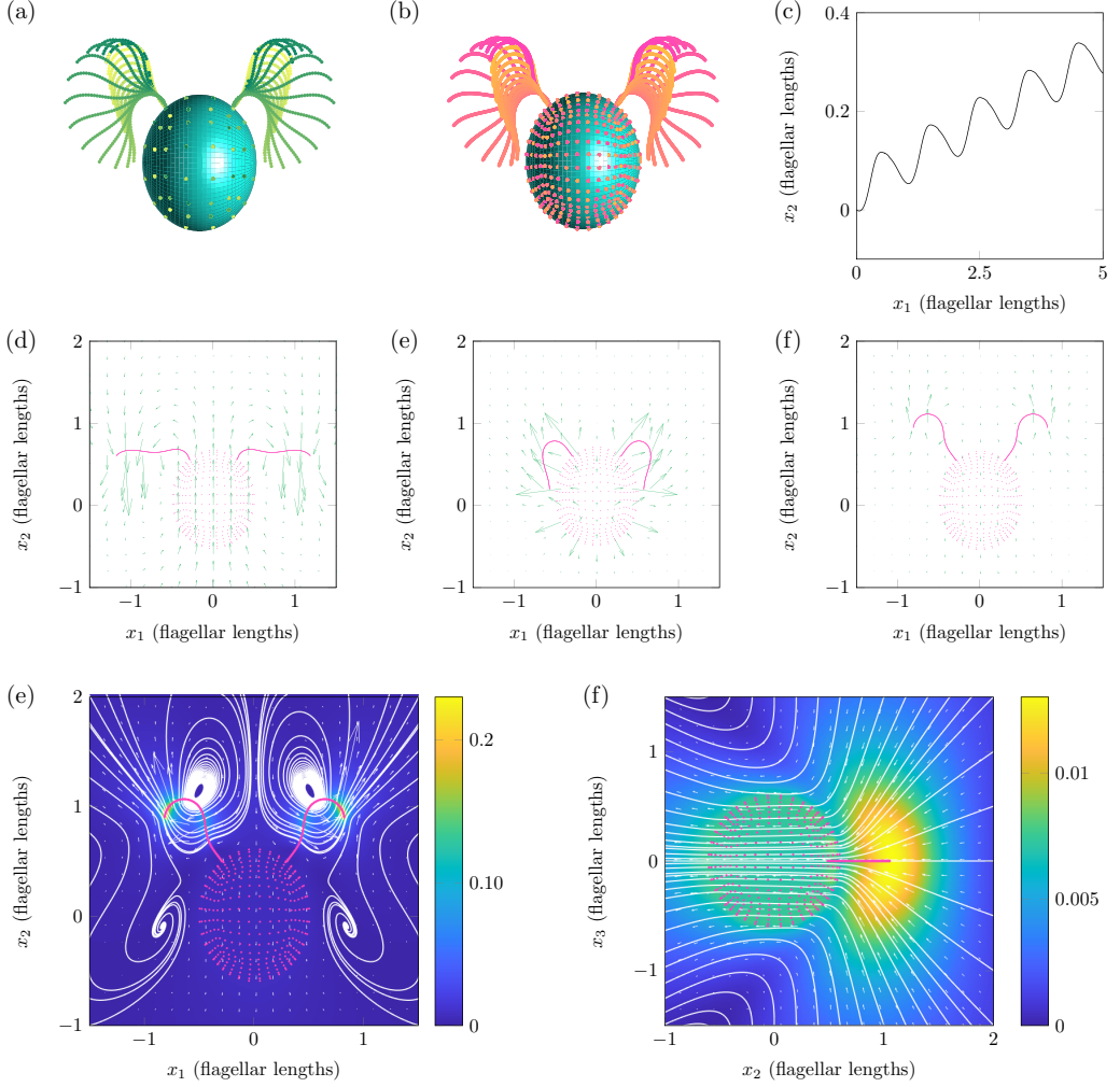
FIG. 1. Computational results for a free-swimming model biflagellate in an unbounded fluid, implemented with the script GenerateSwimmingFigureChlamy.m . Model biflagellate show the beat pattern, visualized via (a) force discretization and (b) quadrature discretization. (c) The x_2 coordinate of the free-swimming cell over five beat cycles, where positive x_2 is the overall swimming direction. The computed flow fields are shown at (d) t = 2\pi/3 , (e) t = 4\pi/3 , and (f) t = 2\pi (three points during the beat cycle). The computed velocity profile with streamlines is shown at t = 0 for cross sections of the (g) (x_1, x_2) and (h) (x_2, x_3) planes.
