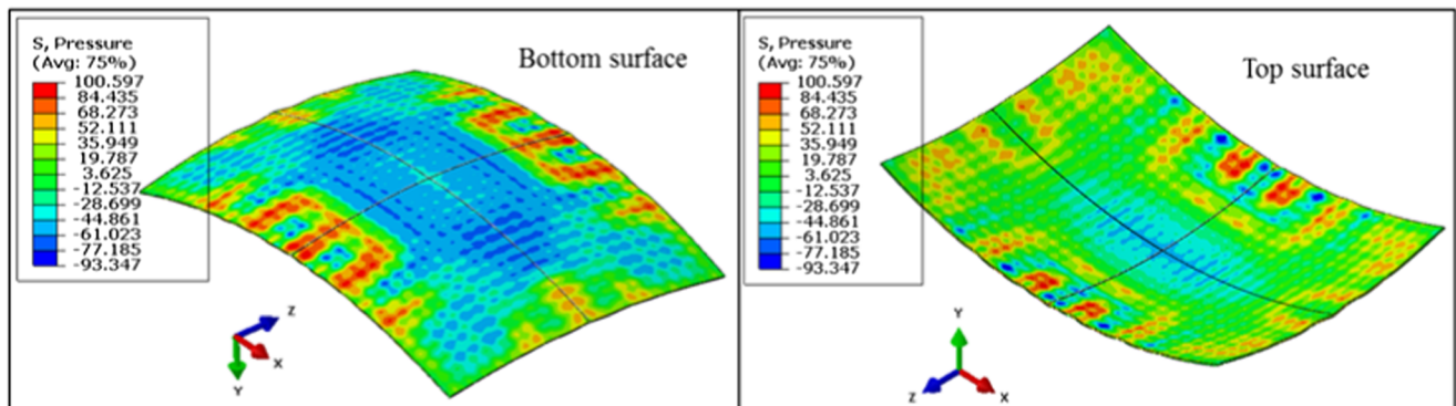
Fig. 11 Pressure distributions on top and bottom surfaces of formed part before springback ( R = 400 mm)
