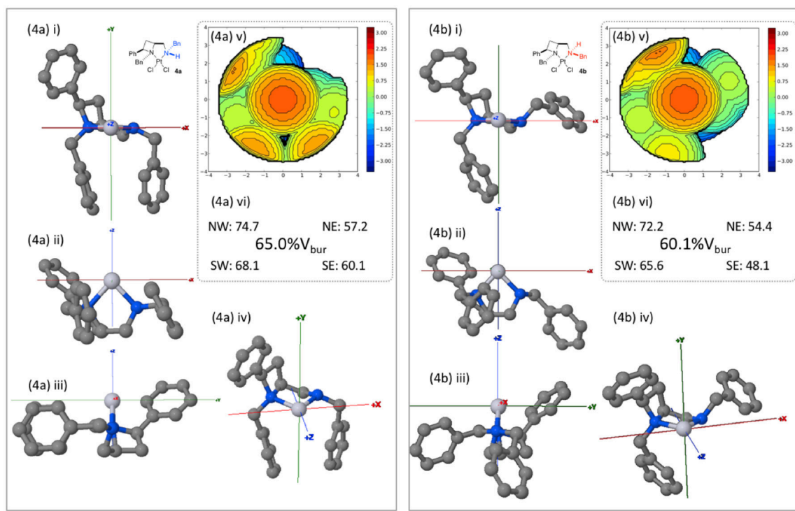
FIGURE 6 | Burried volume analysis of ligand geometries in complexes 4a and 4b , conducted using online tool SambVca 2.0. (i–iv) Various orientations of the considered structures; (v) SambVca-generated %V bur map; and (vi) %V bur and quadrantwise contributions.
