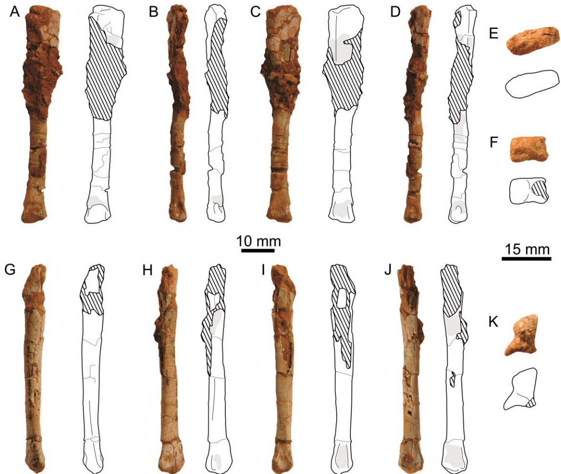
FIGURE 12. Nhandumirim waldsangae gen. et sp. nov. (LPRP/USP 0651). Right metatarsals II ( A-F ) and IV ( G-K ) in ( A and G ) cranial, ( B and H ) lateral, ( C and I ) caudal, ( D and J ) medial, ( E ) proximal and ( F and K ) distal views. Light grey indicates scarred areas, and cross-hatched areas represent broken portions. [planned for page width]
