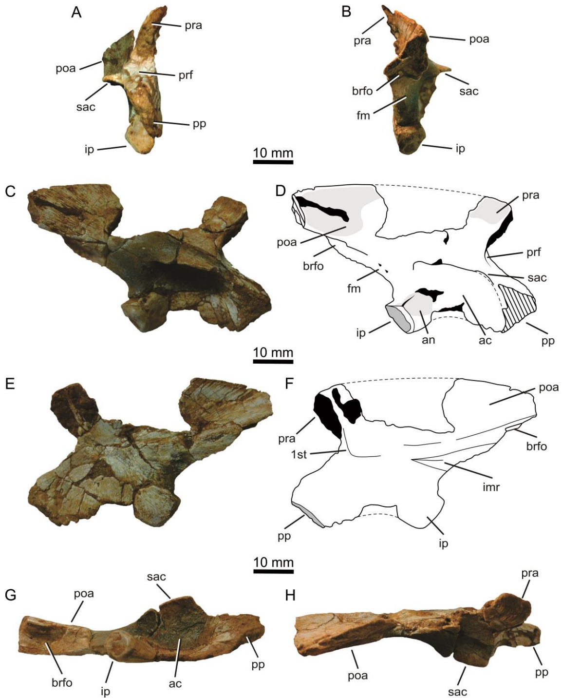
FIGURE 8. Nhandumirim waldsangae gen. et sp. nov. (LPRP/USP 0651). Right ilium in (A) cranial, (B) caudal, (C and D) lateral, (E and F) medial, (G) ventral and (H) dorsal views. D and F are outline drawings of C and E, respectively. Parts in black represent portions still covered by sediment; light gray represents scarred areas; dark gray represents articular facets of the peduncles; dashed lines represent the possible limits of missing parts; cross-hatched areas show broken parts. Abbreviations: 1st,
