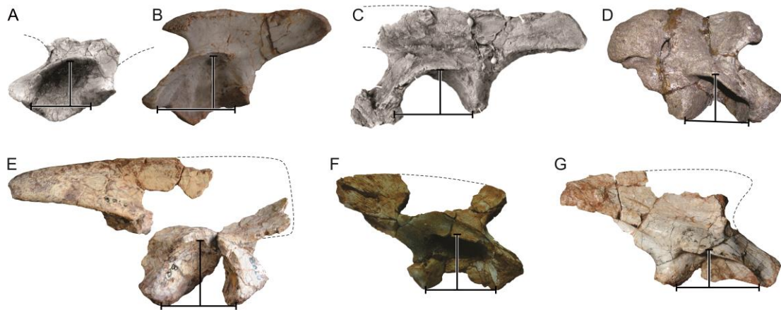
FIGURE 17. Lateral view of several early dinosauriform ilia, showing the depth of the acetabulum. Dashed lines represent the possible limits of missing parts. A , Asilisaurus kongwe (NMT RB159, after Peacock et al., 2013); B , Ixalerpeton polesinensis (ULBRA-PVT059); C , Eocursor parvus (SAM-PK-K8025, after Butler, 2010); D , Herrerasaurus ischigualastensis (PVL 2566); E , Coelophysis bauri (AMNH FARB 2708); F , Nhandumirim waldsangae gen. et sp. nov. (LPRP/USP 0651); G , Saturnalia tupiniquim (MCP-3845 PV). Specimens scaled to the same acetabular length. [planned for page width]
