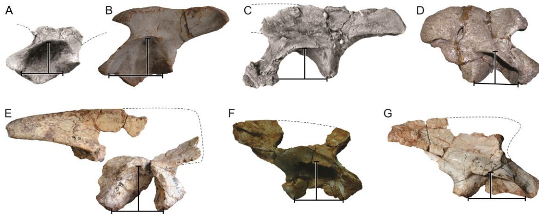
FIGURE 17. Lateral view of several early dinosauromorph ilia, showing the depth of the acetabulum. Dashed lines represent the possible limits of missing parts. A , Asilisaurus kongwe (NMT RB159, after Peacock et al., 2013); B , Ixalerpeton polesinensis (ULBRA-PVT059); C , Eocursor parvus (SAM-PK-K8025, after Butler, 2010); D , Herrerasaurus ischigualastensis (PVL 2566); E , Coelophysis bauri (AMNH FARB 2708); F , Nhandumirim waldsangae gen. et sp. nov. (LPRP/USP 0651); G , Saturnalia tupiniquim (MCP-3845 PV). Specimens scaled to the same acetabular length. [planned for page width]
