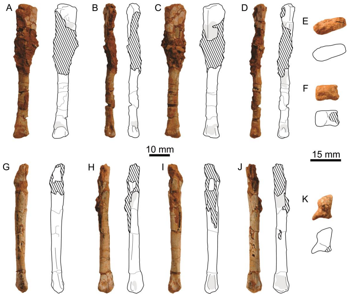
FIGURE 12. Nhandumirim waldsangae gen. et sp. nov. (LPRP/USP 0651). Right metatarsals II (A-F) and IV (G-K) in (A and G) cranial, (B and H) lateral, (C and I) caudal, (D and J) medial, (E) proximal and (F and K) distal views. Light grey indicates scarred areas, and cross-hatched areas represent broken portions. [planned for page width]
