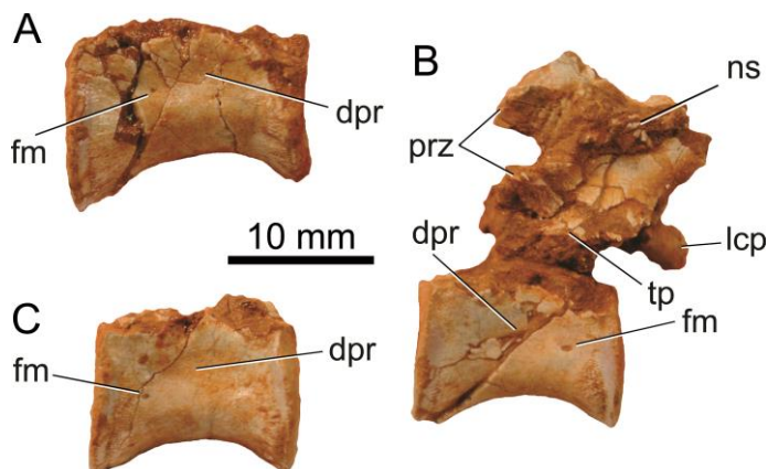
FIGURE 3. Nhandumirim waldsangae gen. et sp. nov. (LPRP/USP 0651). Trunk vertebrae “1”(A), “2” (B) and “3” (C) in right lateral (A) and left lateral (B–C) views.
