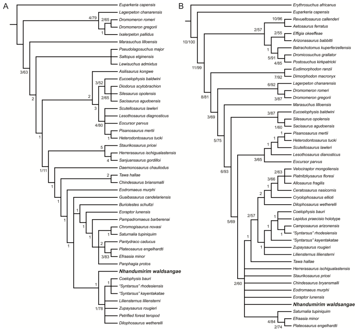
FIGURE 18. Phylogenetic relationships of Nhandumirim waldsangae gen. et sp. nov. (LPRP/USP 0651) among early dinosauromorphs. A , Strict consensus of 48 MPTs found in the analysis of the data matrix of Cabreira et al (2016); B , Strict consensus of 48 MPTs found in the analysis of the data matrix of Nesbitt and Ezcurra (2015). Values at nodes are Bremer support and bootstrap proportions (above 50%). [planned for page width]
