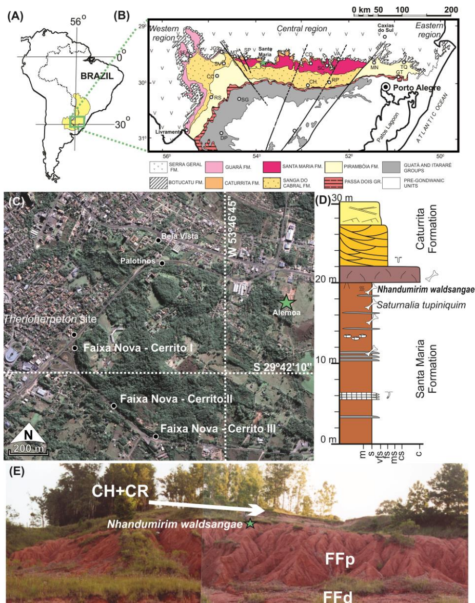
FIGURE 1. Geographic and geologic provenance of Nhandumirim waldsangae gen. et sp. nov. A , map of the Paraná Basin in South America; B , simplified geological map of the central portion of Rio Grande do Sul State (modified from Eltink et al., 2016), indicating Santa Maria (green star); C , location of selected outcrops in the eastern outskirts of Santa Maria (modified from Da Rosa, 2014), indicating the Waldsanga/Cerro da Alemoa site (green star); D , sedimentary log from the Waldsanga/Cerro da Alemoa outcrop, indicating the provenance of the studied specimen and other fossiliferous beds (modified from Da Rosa, 2005); E , photograph of the outcrop, showing the channel and crevasse deposits (CH+CR) of the Caturrita
