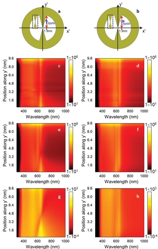
Fig. 6 Schematic representation of the bowtie nanocavity with a vertical (a) and a horizontal emitter (b). Analytical (c, d) and numerical (e, f) \bar{T}_r for the bowtie nanocavity with \theta' = 20^\circ and a vertical (c, e) and a horizontal emitter (d, f) at x' = 2.6 nm and moving along the y' axis. Numerical \bar{T}_r for vertical (g) and horizontal emitter orientations (h).
