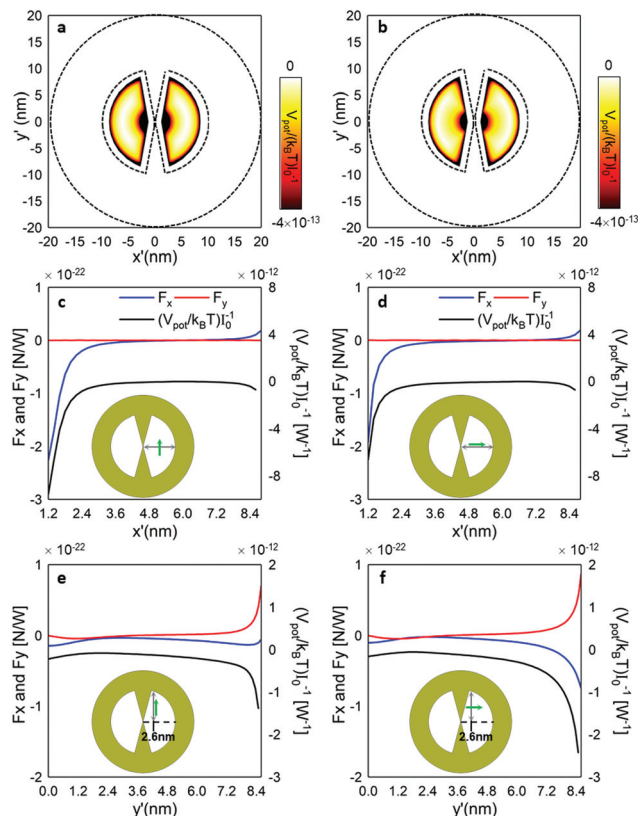
Fig. 7 (a, b) The normalized self-induced trapping potential distribution of a \phi 2 nm colloidal ZnO QD inside a \theta' = 20^\circ nanocavity at the LSP resonant wavelength of 779.2 nm – photoluminescence polarized vertically – (a) and 697.7 nm – photoluminescence polarized horizontally – (b). (c, d) Normalized forces along the x ( F_x ) and y ( F_y ) axes (blue and red lines, respectively) together with the normalized self-induced trapping potential (black line) calculated at the y' = 0 horizontal line as shown in the insets for the photoluminescence polarized vertically (c) and photoluminescence polarized horizontally (d). (e, f) Normalized forces along the x ( F_x ) and y ( F_y ) axes (blue and red lines, respectively) together with the normalized self-induced trapping potential (black line) calculated at x' = 2.6 nm vertical line as shown in the insets for the photoluminescence polarized vertically (e) and photoluminescence polarized horizontally (f).
