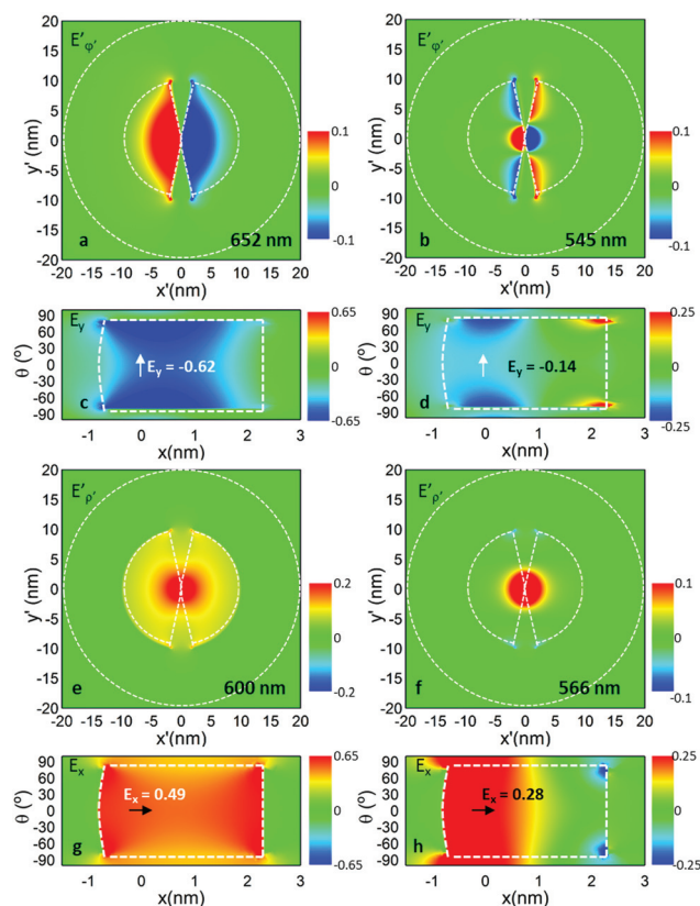
Fig. 4 Electric field distribution E'_\varphi(x', y') and E'_\rho(x', y') of the first two LSP modes for \theta' = 20^\circ under vertical (a, b) and horizontal (e, f) emitter orientations, respectively. Note that the colour scale has been saturated in order to better appreciate the field distribution. The corresponding electric field distributions E_y(x, y) and E_x(x, y) in the transformed space for vertical (c, d) and horizontal (g, h) emitter orientations.
