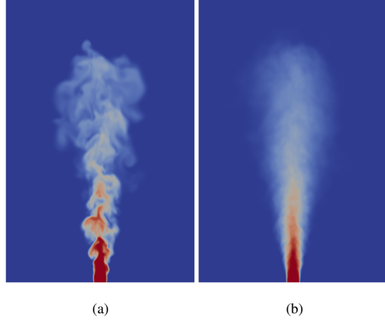
Figure 5: Mass fraction of the injected gas at t=1.2 ms. (a) LES instantaneous field; (b) Ensemble-averaged field over 20 LES realizations;
