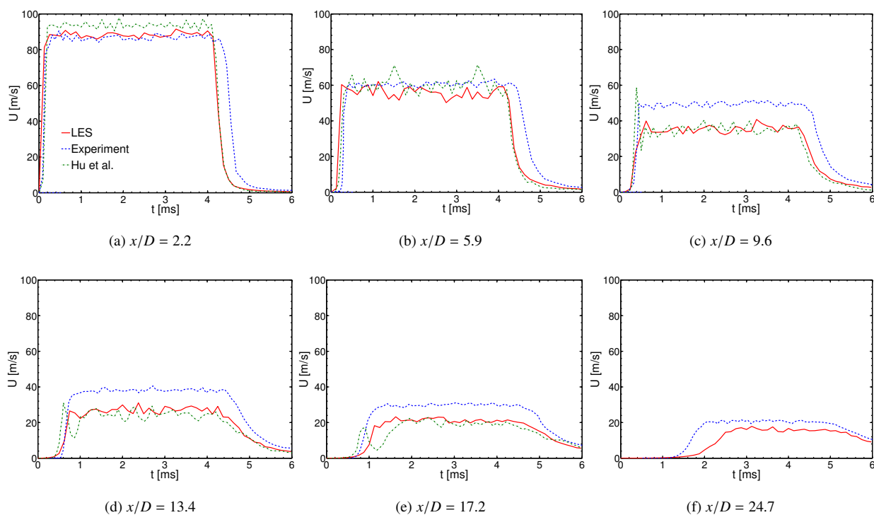
Figure 4: Ensemble-averaged centerline axial velocity at various downstream locations; present prediction, the measurement in the experiments [24] and the results of Hu et al. [19].
