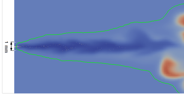
Figure 1: White small spheres are the liquid parcels and their diameter shows the actual diameter of the particles inside the parcel, the green line is iso-counter of the mixture fraction equal to 0.1% and shows the limits of the gas-phase zone of the spray. The diameter of the liquid injector is 0.1 mm and the initial diameter of the gas phase is around 1 mm [6].
