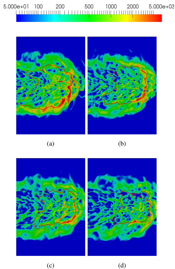
Figure 10: Ensemble average of (\nabla Z_1)^2 ; (a) case 2 at t=1.8 ms; (b) case 3 at t=2 ms; (c) case 4 at t=2.1 ms; (d) case 5 at t=2.3 ms; Each frame shows a domain of 14\text{cm} \times 20\text{cm} . Lines are iso-contour of Z_1 and Z_2 , for more detail see the caption of Fig. 9.
