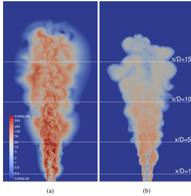
Figure 6: The instantaneous distribution of turbulent kinetic energy at t = 1.2ms . (a) resolved scale kinetic energy, k_{res} ; (b) modeled sub-scale kinetic energy, k_{sgs} ; A logarithmic scale is used.
