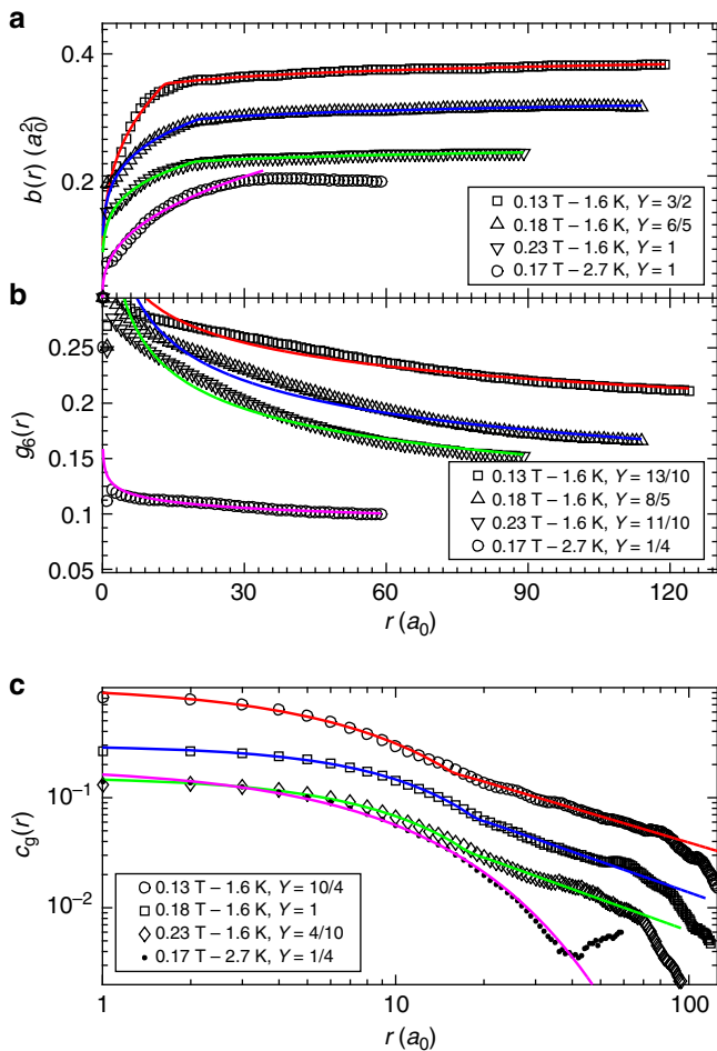
Fig. 8 In-plane correlations deduced by reverse Monte Carlo refinement. Correlation functions calculated from simulated vortex ensembles (open symbols) that reproduce the neutron scattering data in Fig. 7. For clarity curves are offset with a multiplication factor Y . (a) Displacement clarity b(r) = \langle (\mathbf{u}_j - \mathbf{u}_i)^2 \rangle . (b) Hexatic orientational order g_6(r) = \langle e^{i6(\theta_j - \theta_i)} \rangle is fitted with a single algebraic decay \propto r^{-\eta_6} . (c) Translational order c_g(r) = \langle e^{i\mathbf{g} \cdot (\mathbf{u}_j - \mathbf{u}_i)} \rangle and b(r) comprise three regimes in the Bragg glass picture: the Larkin, random manifold and Bragg glass regimes (see text). Here the Larkin regime lies at indiscernibly small length scales and two-part functions fit b(r) and c_g(r) (solid lines) for the three datasets at 1.6 K. For the 0.17 T, 2.7 K dataset, which lies close to the order-disorder line, a single function fits c_g(r) corresponding to the random manifold regime
