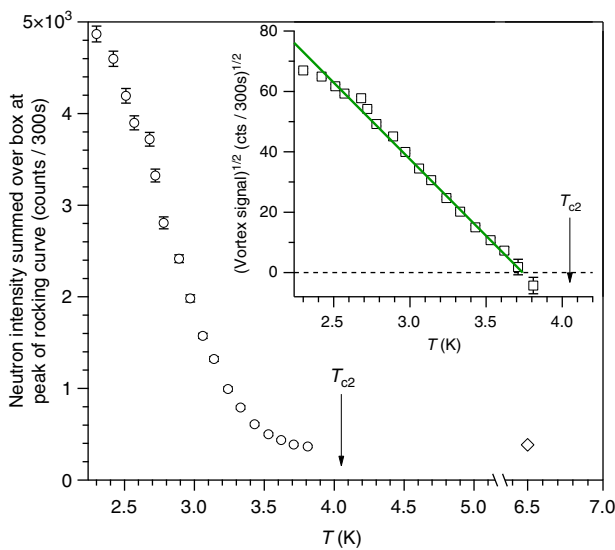
Fig. 6 Temperature dependence at 0.13 T. Neutron scattering from the vortex ensemble is measured on warming, after field-cooling to 2 K. Using the perpendicular field geometry (Fig. 2b), neutron counts are collected at the peak of the rocking curve and summed over a box on the 2D multidetector encompassing the Bragg spot (red box in Fig. 2b). The diamond indicates a background measurement at T > T_c characterising the non-vortex scattering that arises predominantly from the walls of the closed-cycle refrigerator used to cool the sample. Error bars are determined by Poisson statistics. Inset shows the square root of the vortex signal I_p , which is proportional to the vortex form factor h when the field is constant. Negative values of vortex signal, arising from the background subtraction, are indicated by plotting \text{sgn}(I_p)\sqrt{|I_p|} . Green line is a guide to the eye showing a linear variation, as expected from mean field theory in the vicinity of a phase transition
