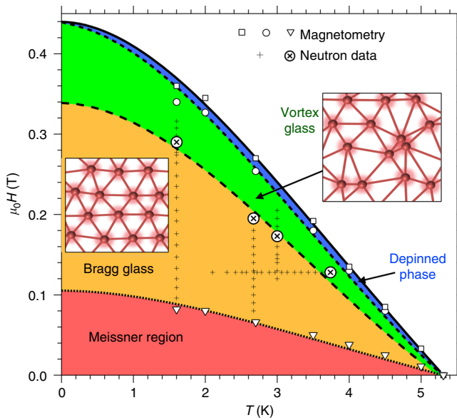
Fig. 1 Phase diagram. Vortex phase diagram for our vanadium single crystal from magnetometry and neutron scattering experiments. Superconductivity appears below the upper critical field B_{c2}(T) (squares and solid line), with vortices forming between B_{c2}(T) and the lower critical field B_{c1}(T) (triangles and dotted line). The critical current j_c is observed to collapse in a region close to B_{c2}(T) (circles and short-dashed line). This collapse indicates that vortices are detaching from their pins. Vortex correlations are probed directly by neutron scattering. Plus signs mark the temperatures and fields where neutron scattering data were collected. The disappearance of neutron diffraction peaks (crosses in circles) marks the vortex order-disorder transition H_{dis}(T) . Short-dashed and long-dashed lines are fits based on different types of Lindemann criteria 23 described in the text. The insets schematically illustrate the vortex phases either side of the order-disorder line. Intriguingly, the peak effect is not located at the order-disorder line. Instead it is observed close to the depinning line
