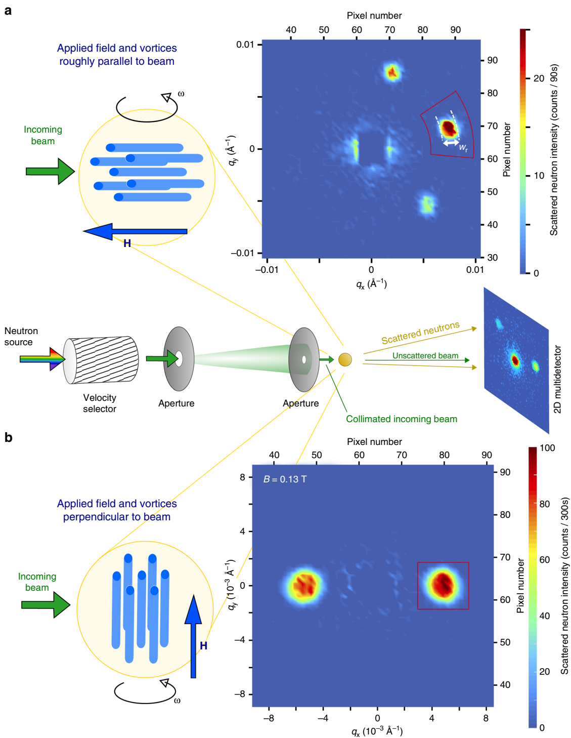
Fig. 2 Neutron scattering geometries. Small-angle neutron scattering (SANS) instruments are usually pinhole cameras with small apertures to tightly collimate the incoming neutron beam. The magnetic field profile presented by vortices in the sample diffracts neutrons. Rocking curves are collected by rotating the sample, field and vortices together through the Bragg condition. Two experimental geometries may be used, exploiting the significantly better instrument resolution in the direction probed by the rocking curve: (a) The applied magnetic field and vortices are orientated roughly parallel to the neutron beam. Here the rocking curve is most sensitive to correlations along the vortices. A typical image of the 2D SANS multidetector at the peak of the rocking curve of the right Bragg spot is shown. The rotation axis for this rocking curve is indicated by \omega . The unscattered neutron beam in the centre of the image at \mathbf{q} = 0 is blocked by a beamstop. (b) The rocking curve probes correlations in the plane of the vortices when the applied magnetic field and vortices are orientated perpendicular to the neutron beam. The detector image shows the peak of the rocking curve of the right spot at 0.13 T
