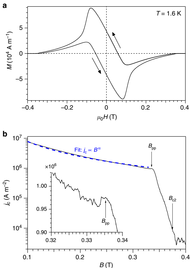
Fig. 3 Magnetometry at 1.6 K. a M(H) loop for our vanadium single-crystal with H \parallel [111] . b Critical current density j_c calculated from the width \Delta M of the magnetisation loop. j_c(B) decreases monotonically except for a small peak, labelled B_{pp} , observed just before the sharp downturn where thermal fluctuations start depinning vortices. The dashed line is a fit to an algebraic decay j_c \propto B^\alpha . Fitted value of \alpha = -1.7 . Inset is a magnification of the region around B_{pp}
