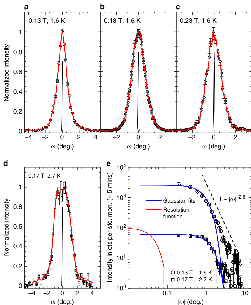
Fig. 7 Neutron scattering in perpendicular field geometry. In the perpendicular field geometry (Fig. 2b), rocking curves probe correlations in the plane of the vortices. a–d Rocking curves of the first order diffraction peak at four selected points in the phase diagram, collected with long counting times to afford high quality data for reverse Monte Carlo refinement. Backgrounds measured at zero field have been subtracted. Ordinate axes are normalised for comparison. In reverse Monte Carlo refinement, simulated vortices are displaced using a Monte Carlo method until the experimental rocking curve (circles) is reproduced (red lines). Black lines indicate instrument resolution. e Rocking curves of a and d on logarithmic axes. Dashed line is a guide showing an algebraic decay. Algebraic tails are expected from the Bragg glass picture. Gaussian fits (blue lines) are drawn for comparison
