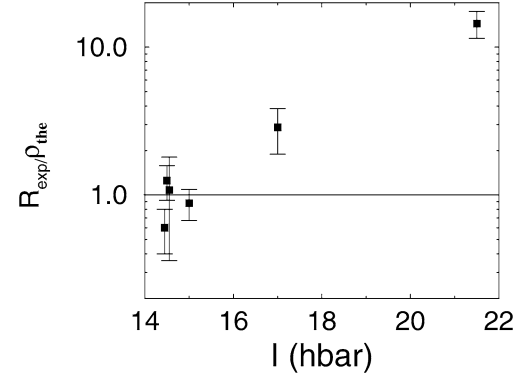
Fig. 2. The ratios of experimentally measured isomeric ratios and the calculated values using the sharp cutoff approximation. For details see the text.
