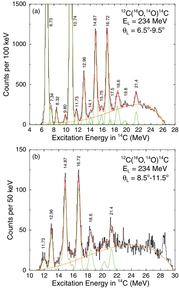
FIG. 1. (Color online) The ^{14}\text{C} excitation energy spectra fitted with Gaussian peaks, whose centroids are indicated, and a smooth background. The peaks ranging from 6.73 to 21.4 MeV represent the ^{14}\text{C} states populated in the two-neutron transfer reaction ^{12}\text{C}(^{16}\text{O}, ^{14}\text{O})^{14}\text{C} . The angular range of the Q3D acceptance aperture is indicated. In (b) the magnetic-field settings of the Q3D have been chosen to emphasize the higher-excitation-energy region. The feature at 28.4 MeV is not an excited state, but rather an edge effect at the low-energy side of the detector.
