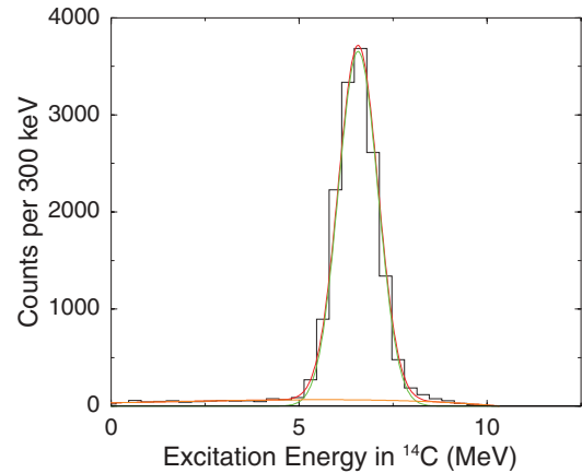
FIG. 5. (Color online) The 6.73 MeV ^{14}\text{C} state populated in the ^{12}\text{C}(^{16}\text{O},^{14}\text{O})^{14}\text{C} reaction. The spectrum is obtained after the coincident detection of the ^{14}\text{C}^* , in the DSSSD array, with the ^{14}\text{O} ejectile, in the Q3D. The data is fitted with a simulated peak line-shape and a smooth background.
