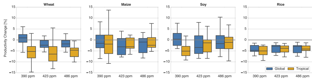
Figure 4. As figure 2 top panel, but for extreme low yields with a return period of 10 years or higher. Extreme low yields are derived as mean over the <10% quantile per warming level and GCM-GGCM pair (45–50 years, see table S2). Relative changes are derived relative to the extreme low yields of the reference period.
