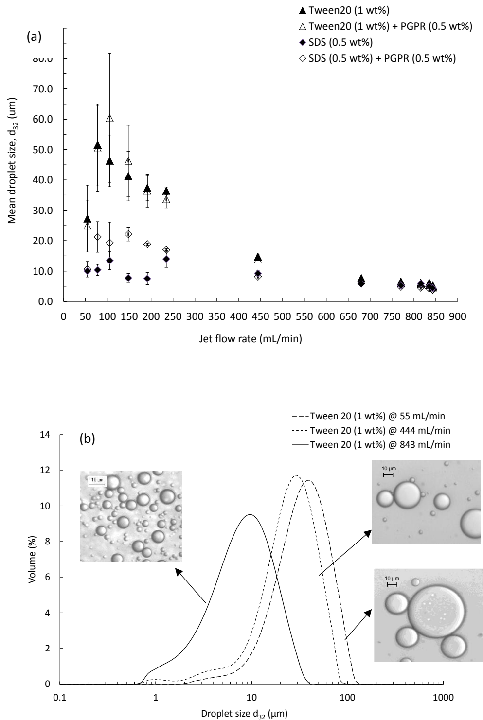
Figure 2: Effect of varying feed flow rate on emulsion (a) drop size and (b) size distribution from mixhead MH-1. Sunflower oil concentration was 5% (v/v).
