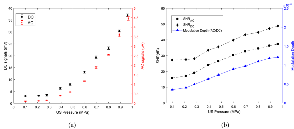
Fig. 4. Influence of varying UST pressure on light source inside the phantom increases (a) Acousto-optic (AC) signals and intensity of light source (DC) and; (b) Modulation depth and SNR of the received AC and DC signals.
