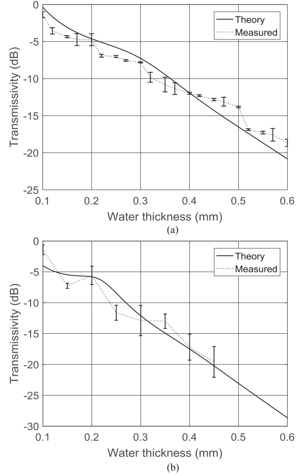
Fig. 5. Calculated and measured transmissivity of pure water film as a function of water thickness at (a) 150 GHz and (b) 300 GHz at 23 °C.
