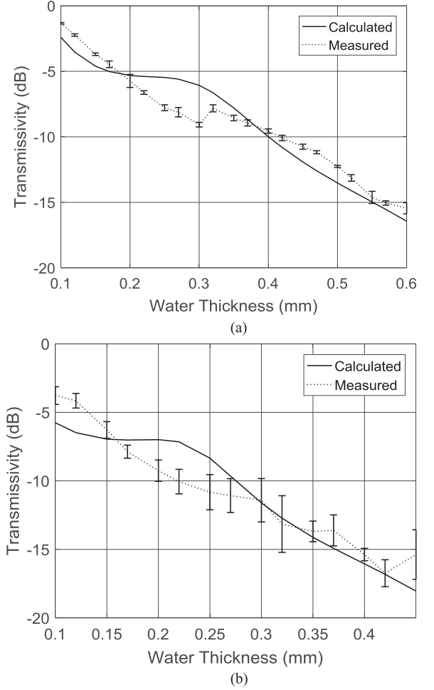
Fig. 7. Calculated and measured transmissivity through a film of water contaminated with salt, with salinity of 3.5% as a function of uniform thickness at (a) 150 GHz and (b) 300 GHz at 23 °C.
