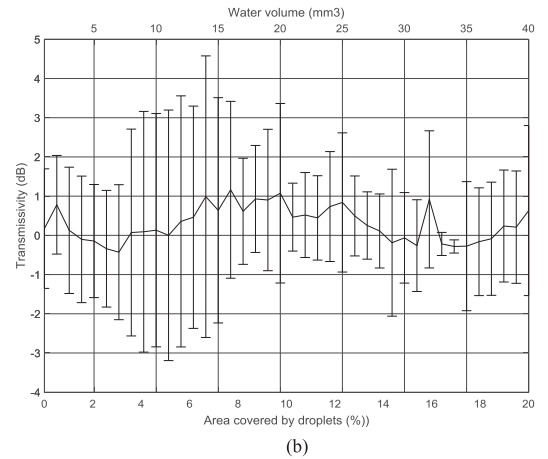
Fig. 16. Transmissivity through pure water droplet screen at 300 GHz. (a) Measured transmissivity (b) average transmissivity.
