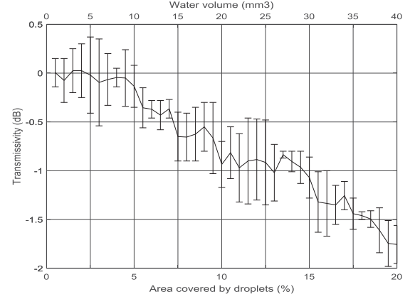
Fig. 15. Transmissivity through randomly distributed droplets at 150 GHz.
