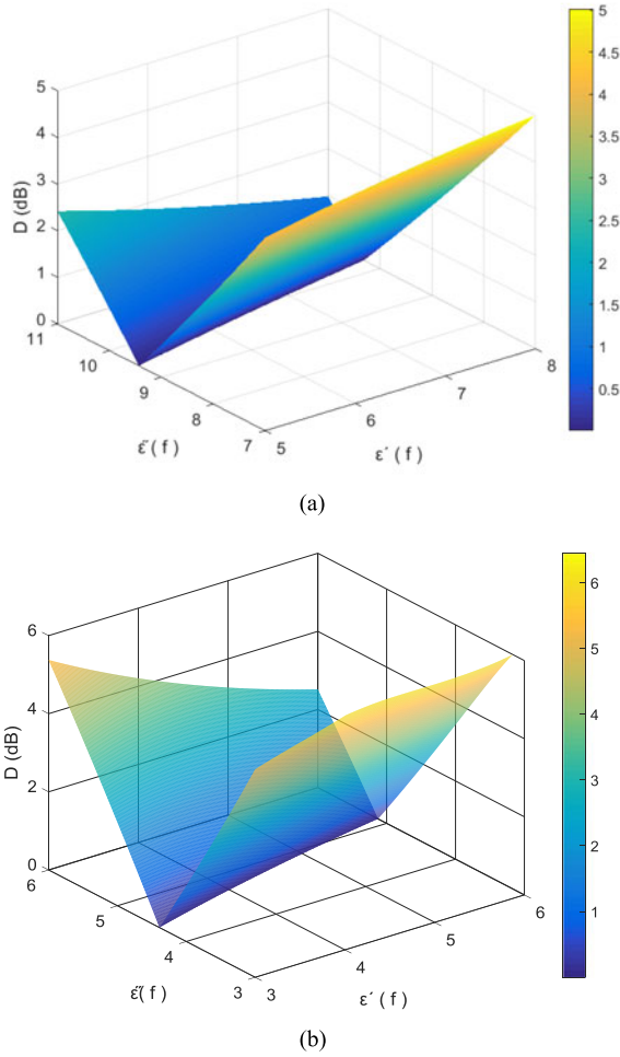
Fig. 4. Deviation between calculated and measured transmissivity at (a) 150 GHz and (b) 300 GHz.
