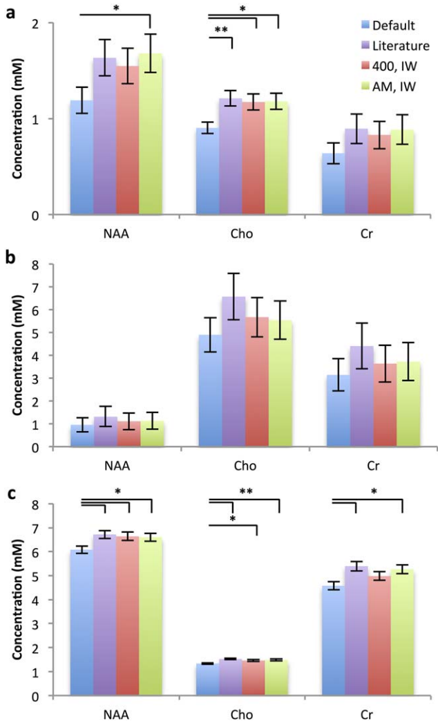
FIGURE 4: Mean \pm standard error metabolite concentrations (mM) in (a) pilocytic astrocytoma, (b) medulloblastoma, and (c) normal brain estimated at short-TE. Metabolite concentrations are corrected for relaxation effects using either default TARQUIN relaxation correction; literature T 2 values; a metabolite T 2 of 400 msec and a patient measured water (IW) T 2 ; or the average metabolite (AM) T 2 for that tissue type and IW T 2 . * P < 0.05 , ** P < 0.01 .
