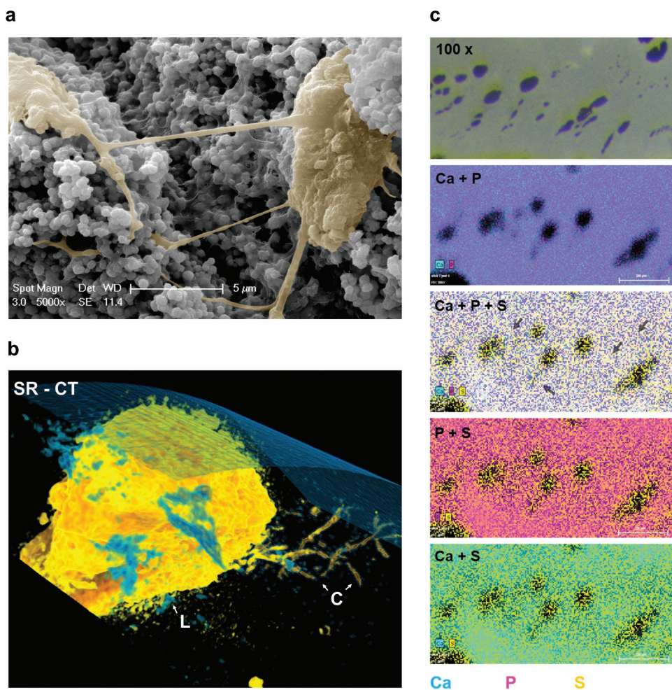
Figure 6. Development of bone cells in constructs. a) SEM images of cells in constructs after 12 months of culture, showing cells embedded in the significantly mineralized matrix. The main cellular structure in a has been false-colored to allow a better visualization. There are many podocytes embedded in the heavily mineralized matrix. Cells communicate through extensive projections. b) Synchrotron radiation computed tomography illustrating a typical osteocyte lacuna (L) with emerging canaliculi (C) that branch into the tissue. c) XRF maps based on S, Ca, P showing network-like structures throughout the matrix and connecting adjacent lacunar-like structures (arrows). Scale bars = 200 \mu\text{m} .
