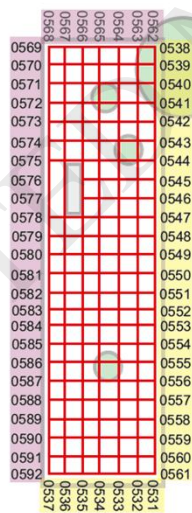
Fig. 4. Known mass grave (left) and potential mass grave (right). Ground-penetrating radar survey profile codes (Yellow = 250 MHz, Purple = 500 MHz). Modified from [41].
