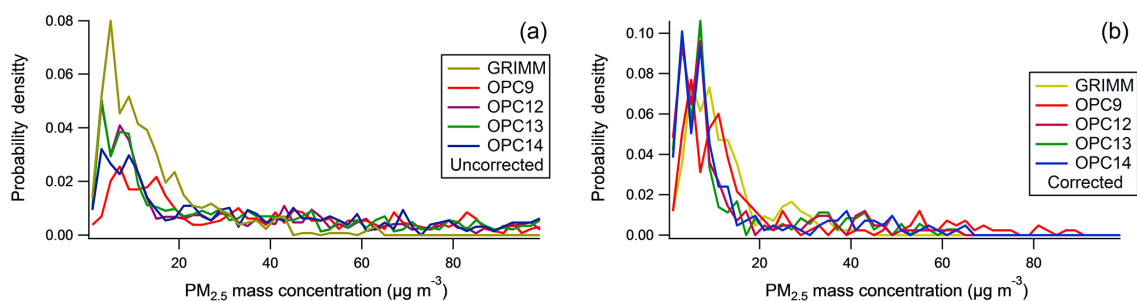
Figure 9. Histogram of measured PM 2.5 concentrations by the GRIMM PAS 1.108 and the four OPC-N2s for January. The uncorrected OPC-N2 concentrations are shown in panel (a), while panel (b) shows the RH-corrected OPC-N2 concentrations.
