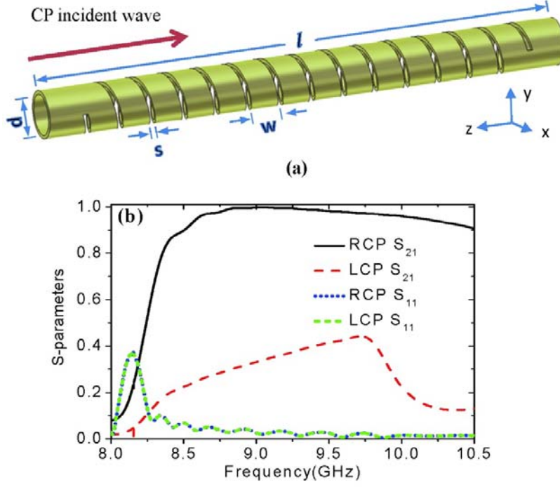
FIG. 1. (a) Schematic diagram of the proposed HTW. The geometric parameters of the HTW are: diameter d = 21.6 mm, metallic copper thickness t = 0.5 mm, slit width s = 4 mm, metallic width w = 15 mm, lattice constant a = s + w = 19 mm, and the number of turns n = 14 , which corresponds to a length of l = 290 mm. (b) Simulated transmission S_{21} and reflection S_{11} for LCP and RCP incident waves.
