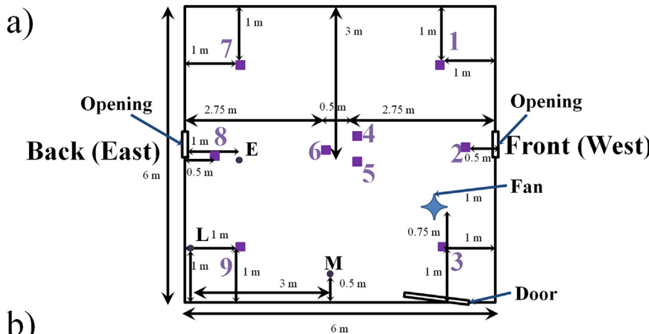
Fig. 3. Tracer gas set-up showing locations of: a) tracer gas inlet pipes (purple squares, 1–9; 1–5 and 7–9 at 3 m above floor level, #6 at ground level), K30 CO 2 sensors (E/L/M, position within 0.1 m), openings (door shown open but closes flush with the wall) and mixing fan (blue cross). b) Photos showing K30 sensors (red circles): Low sensor (L), East sensor (E) and Middle sensor (M). (For interpretation of the references to colour in this figure legend, the reader is referred to the Web version of this article.)
