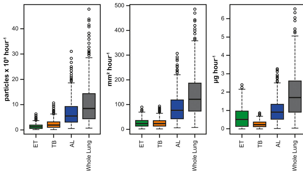
Fig. 4 Hourly dose of outdoor aerosols in the human respiratory system from data from the traffic site, by number (left panel), surface area (central) and mass (right panel)
