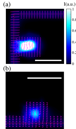
FIG. 4. (color online). The hybrid states for (a) localization A and (b) localization B. The magenta arrows are the normalized Poynting vectors. The white scale bar corresponds to the wavelength in vacuum.
