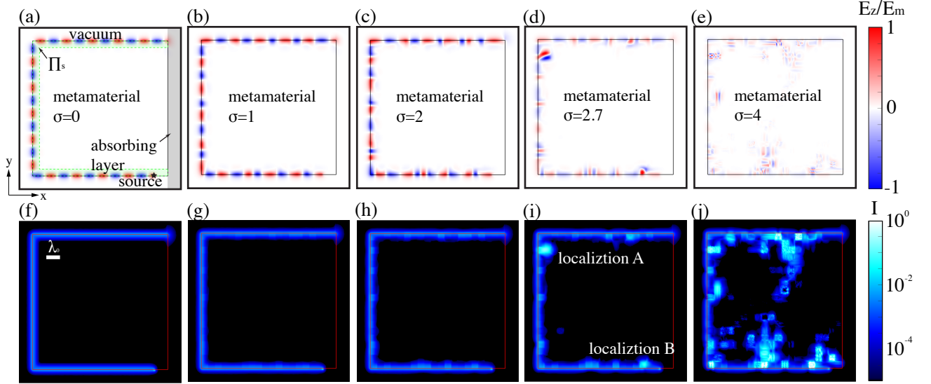
FIG. 2. (color online). (a-e) Normalized E_z in the disorder-perturbed metamaterial for different values of \sigma . (f-j) The corresponding intensities of the field I = |\mathbf{E}|^2 for different values of \sigma .
