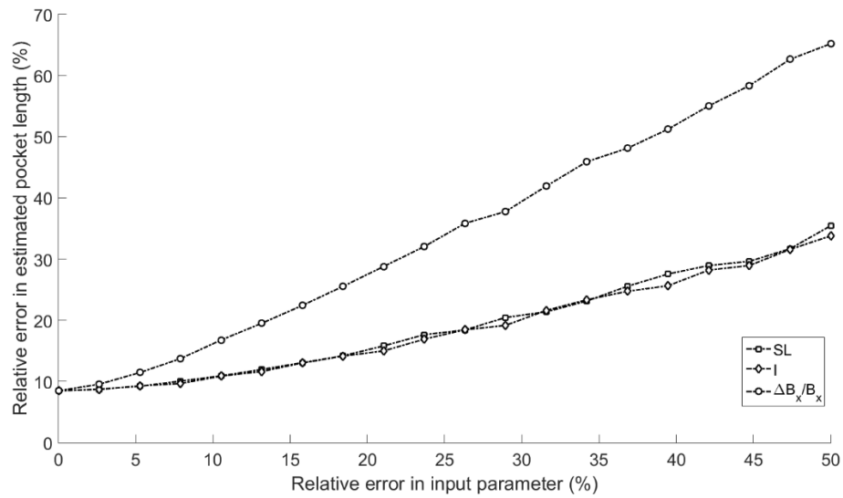
Figure 13 Plot of the network sensitivity to the input parameters S , I and \frac{\Delta B_x}{B_{x_0}} . Results are averaged over training, validation and test sets.
