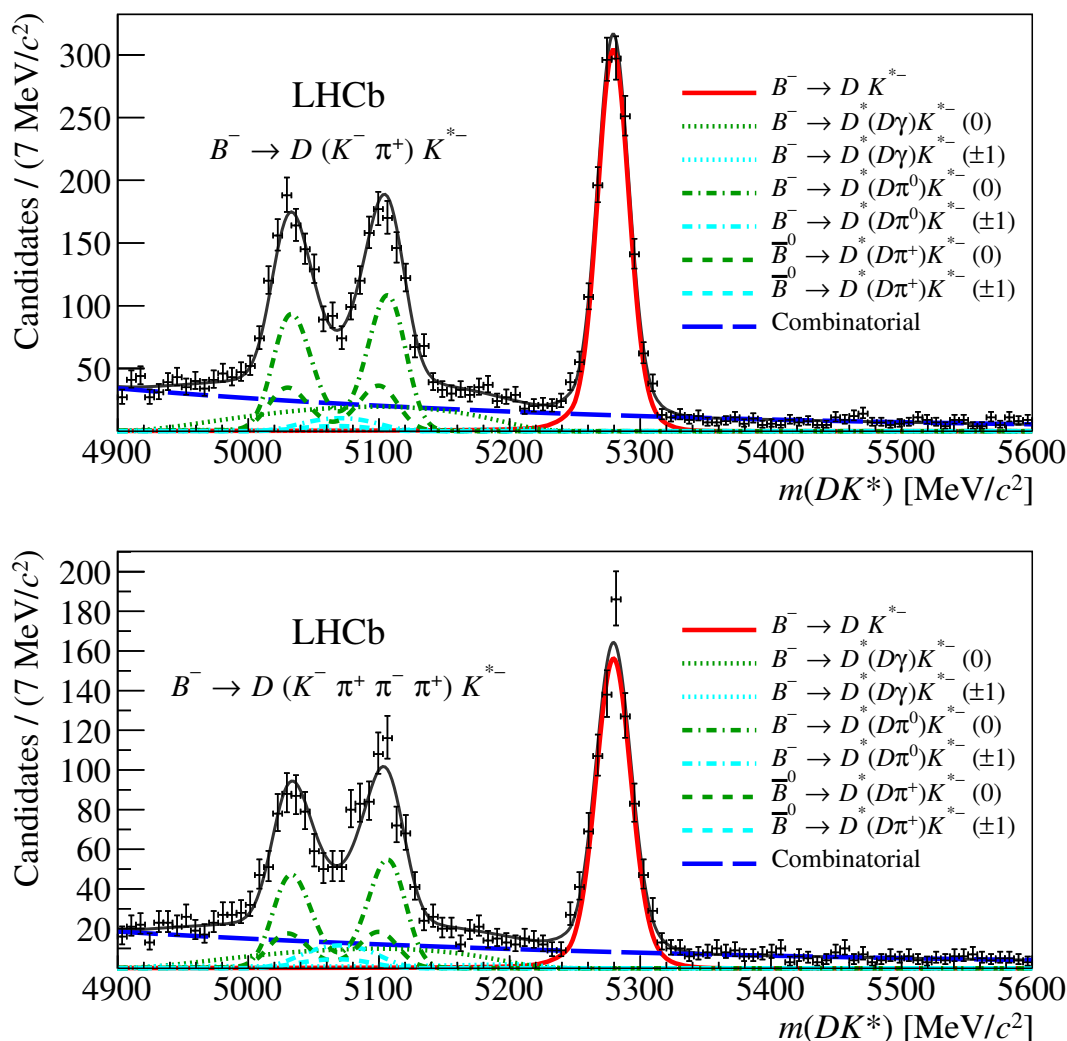
Figure 1. Invariant mass distribution with the fit result superimposed for the favoured B^- \rightarrow D(K^- \pi^+) K^{*-} decay mode (top), and B^- \rightarrow D(K^- \pi^+ \pi^- \pi^+) K^{*-} decay mode (bottom), using Run 1 and Run 2 data combined. The labels 0 and \pm 1 correspond to the helicity state of the D^* meson.
