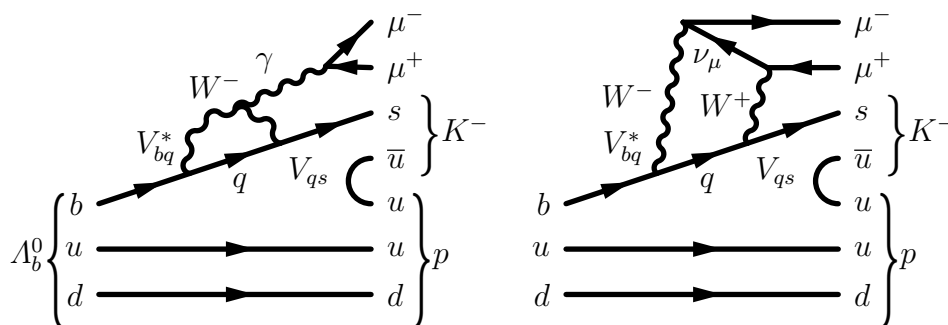
Figure 1. Diagrams for the decay \Lambda_b^0 \rightarrow pK^- \mu^+ \mu^- , in which V_{bq} and V_{qs} are CKM matrix elements and q represents one of the three up-type quarks u, c or t , the t -quark contribution being dominant. The u\bar{u} pairs originate from the hadronization process.
