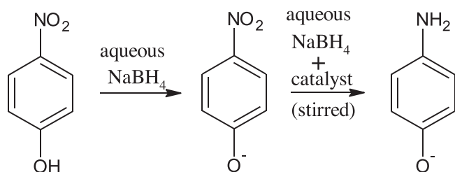
Scheme 1. Reaction scheme of 4-nitrophenol reduction by \text{NaBH}_4 .
