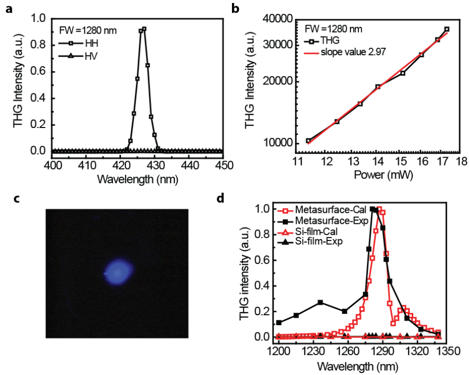
Figure 4. Characterization of third harmonic generation from silicon metasurface. (a) For linearly polarized (TM:H) fundamental waves at wavelength of 1280 nm which is normally incident onto the silicon metasurface, the spectra of THG with both same (H-H) and perpendicular polarization state (H-V) compared to that of the FW are measured. The THG signal for H-H measurement is much stronger (~ eight times) than that for the H-V configuration; (b) Power dependence of the THG intensity (open squares) for the H-H measurement. The result shows a cubic dependence (solid line) with slope value: ~ 3, which verifies the third order nonlinear optical process; (c) Typical THG radiation captured by colour CCD camera; (d) Measured ('Exp') THG spectra agree well with and calculated ('Cal') ones for both silicon planar film and metasurface. The measured giant THG enhancement occurs at wavelength of 1280 nm, which agrees with calculated peak THG value for FW at wavelength of 1287 nm.
